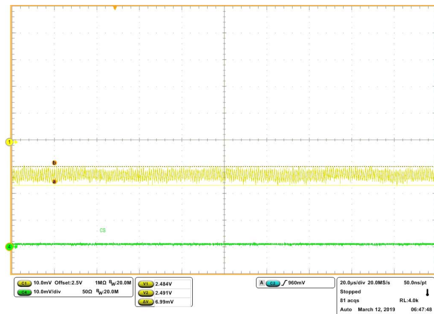
Figure 31. Output Ripple at No Load, <7.0\text{mV}_{\text{P-P}}
