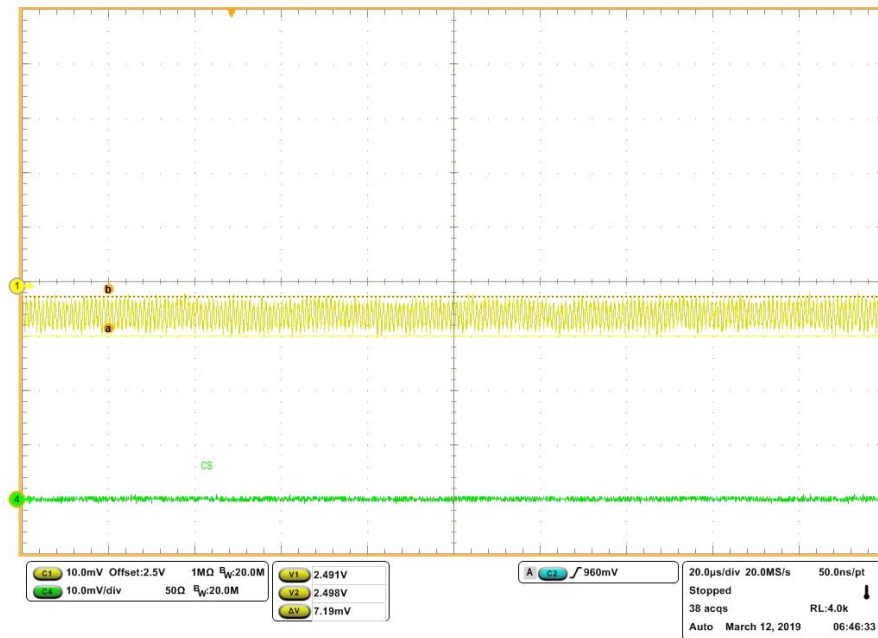
Figure 30. VCCO 2.5V Output Ripple at No Load, <7.19\text{mV}_{\text{P-P}}
