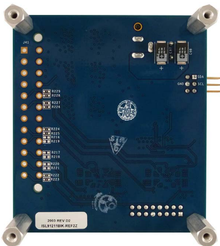
Figure 42. ISL91211BIK-REFZ Bottom
