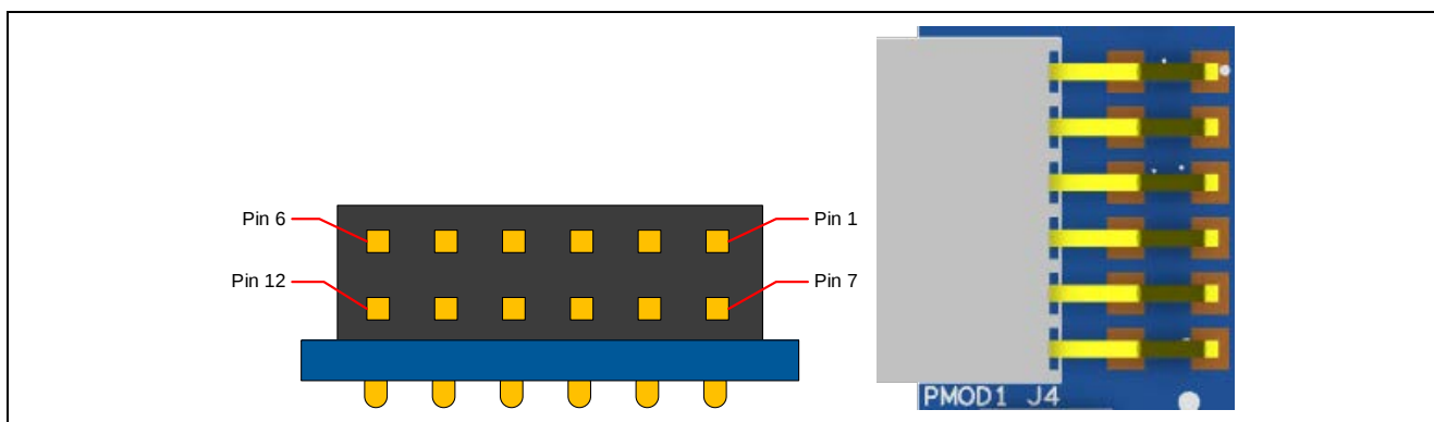
Figure 8. Pmod 1 Connector
