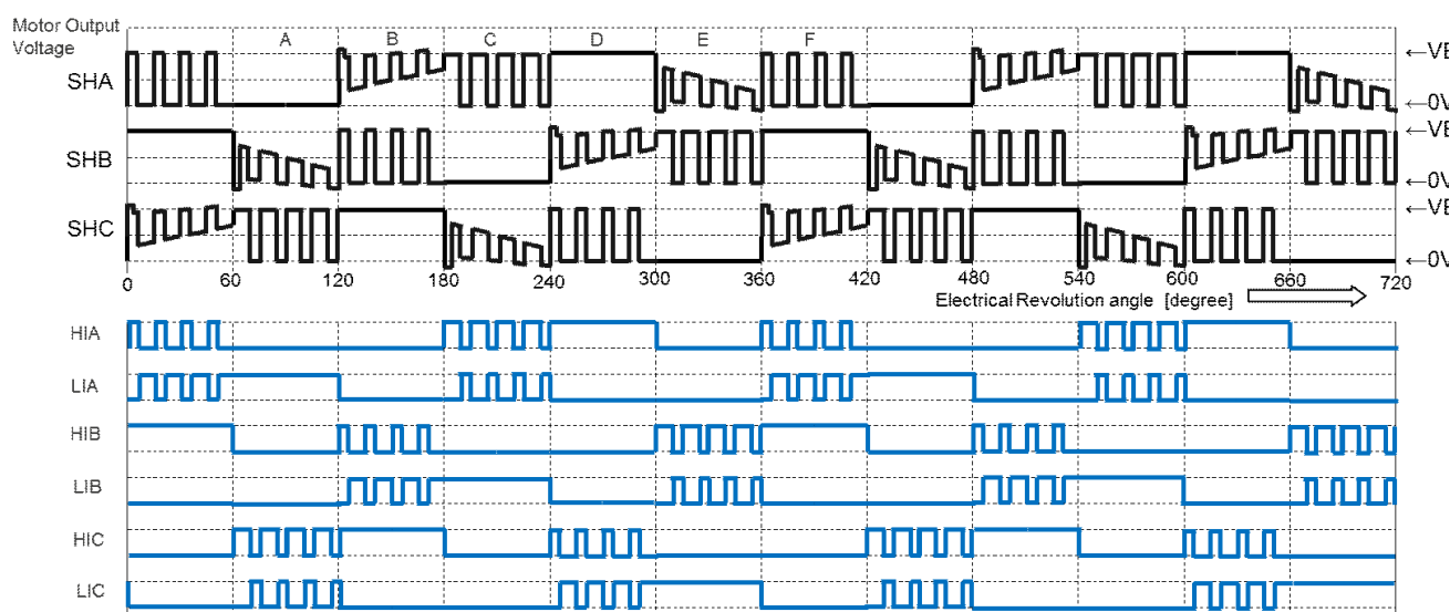
Figure 38. Typical Six Step Trapezoidal Driving Scheme
