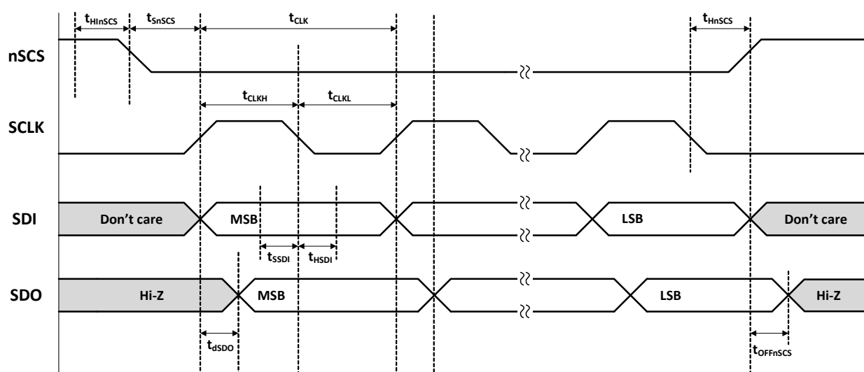
Figure 42. Timing Diagram
