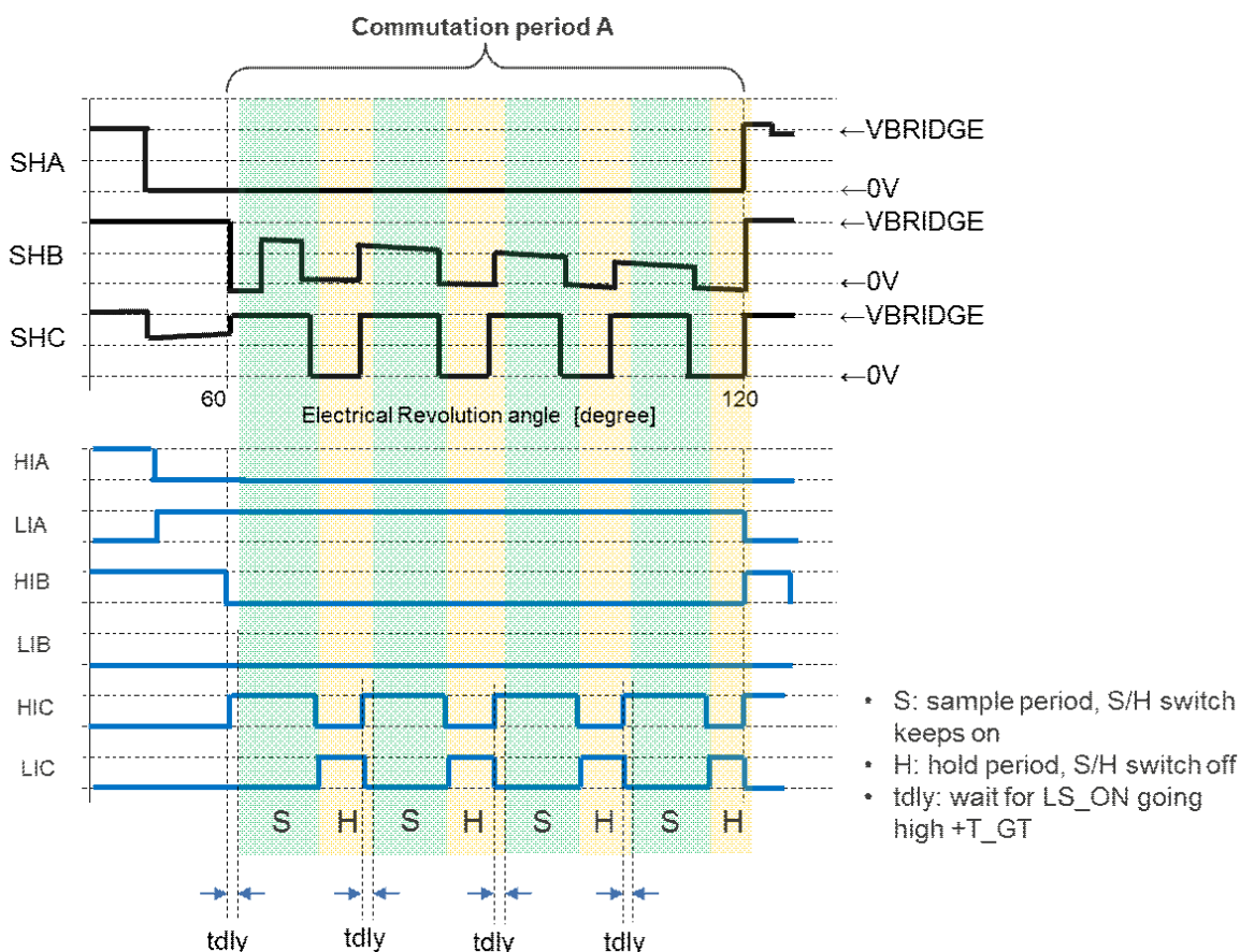
Figure 39. S/H Timing Within Commutation Period A
