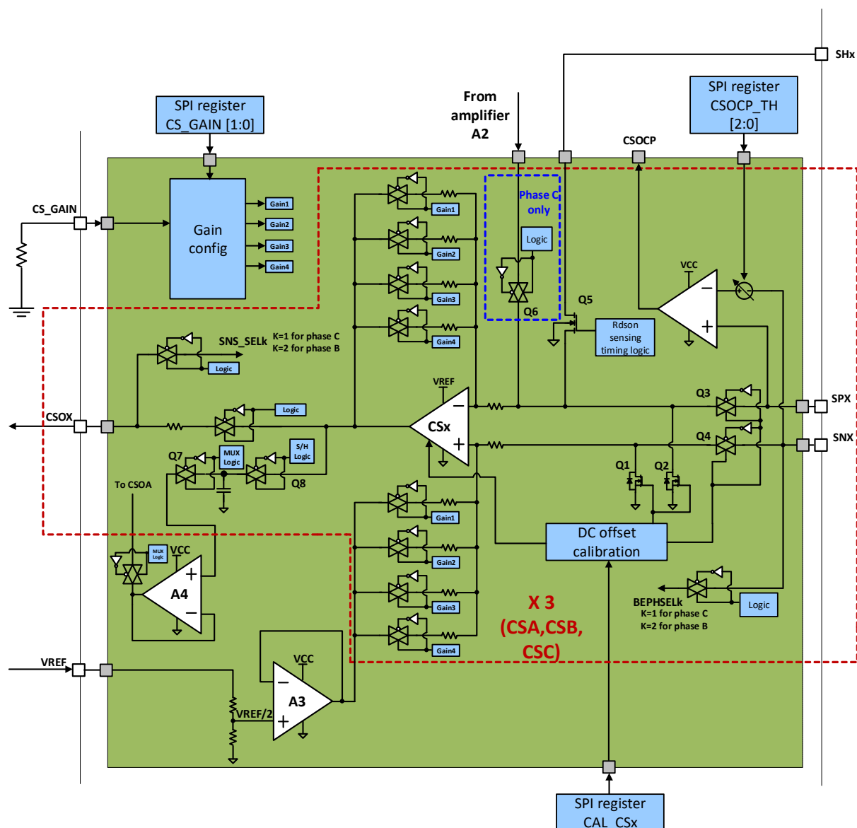
Figure 37. Detailed Block Diagram of CSA, CSB, and CSC Amplifiers
