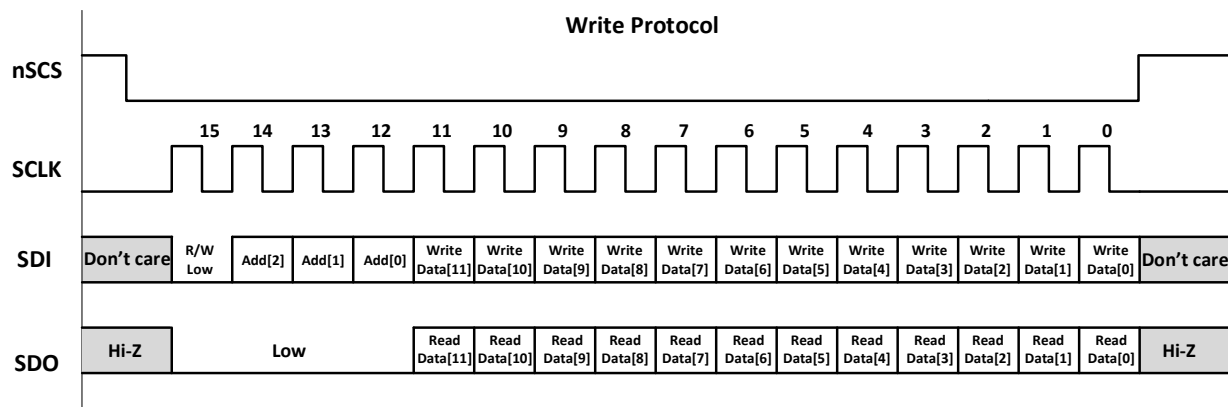
Figure 40. Write Protocol
