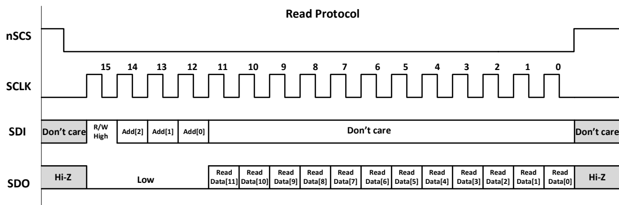
Figure 41. Read Protocol
