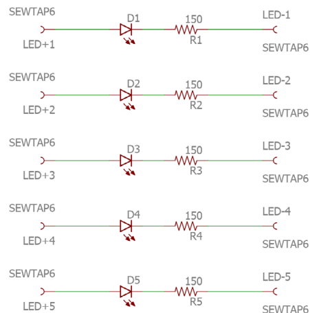
LilyPad LEDs
