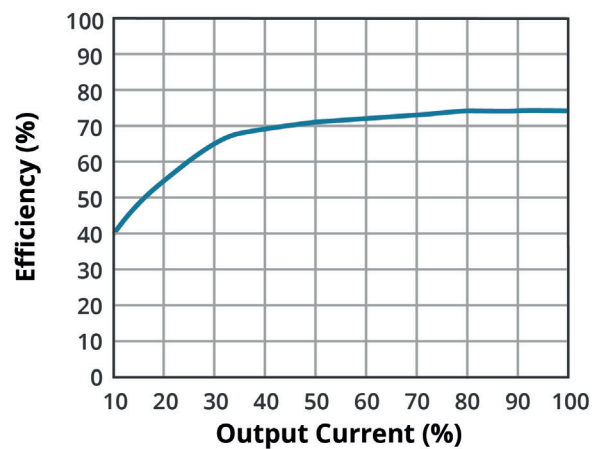
EFFICIENCY VS OUTPUT LOAD ( V_{in} = 12\text{ Vdc} ) PRME1-S24-S5-M
