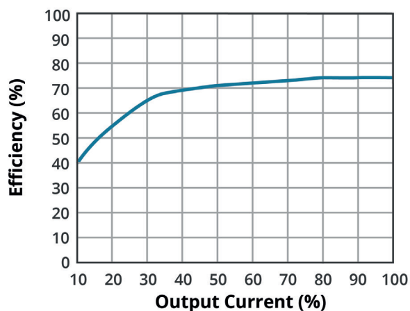
EFFICIENCY VS OUTPUT LOAD ( V_{in} = 12\text{ Vdc} ) PRME1-S12-S5-M
