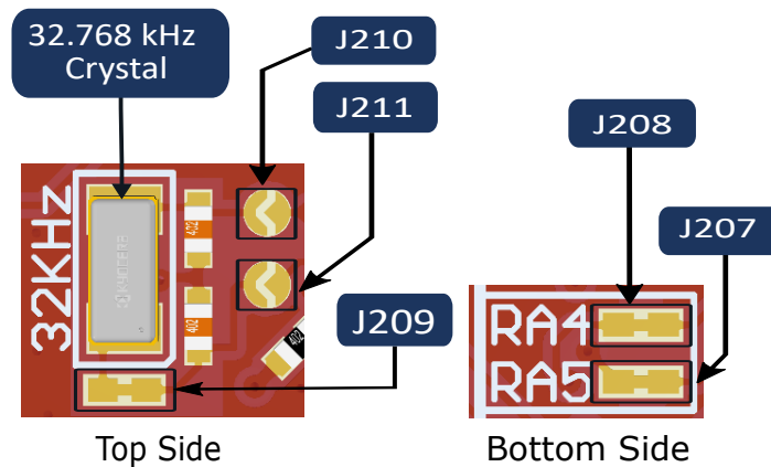
Figure 4-4. Crystal Connection and Cut Straps
