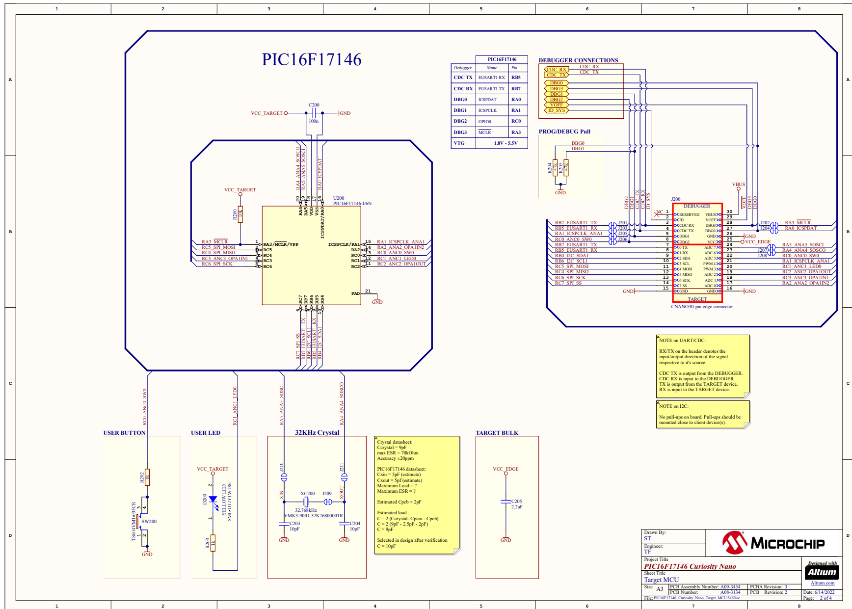
Figure 7-1. PIC16F17146 Curiosity Nano MCU Schematic
