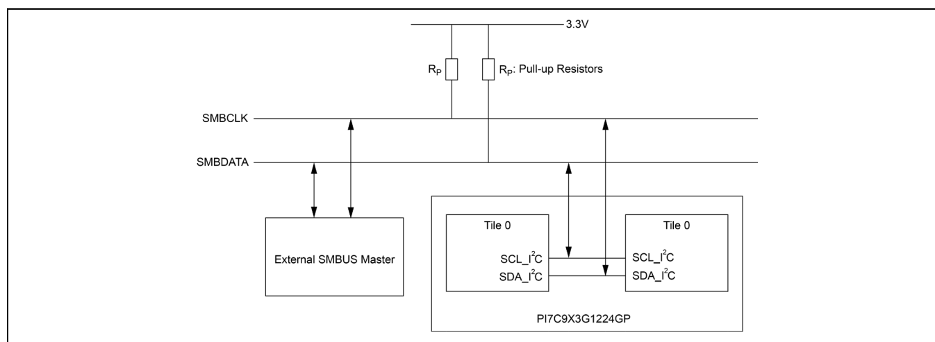
Figure 5-1 SMBus Architecture Implementation
