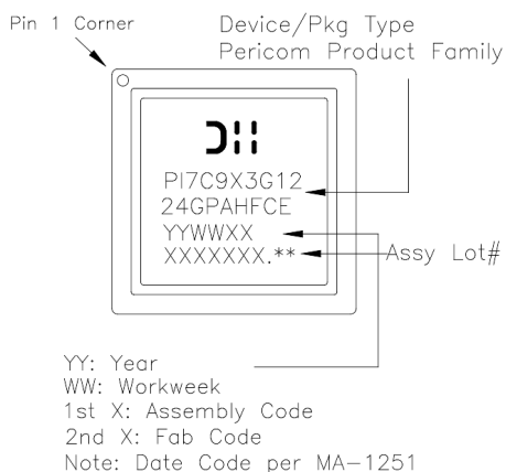
Figure 14-2 Part Marking
