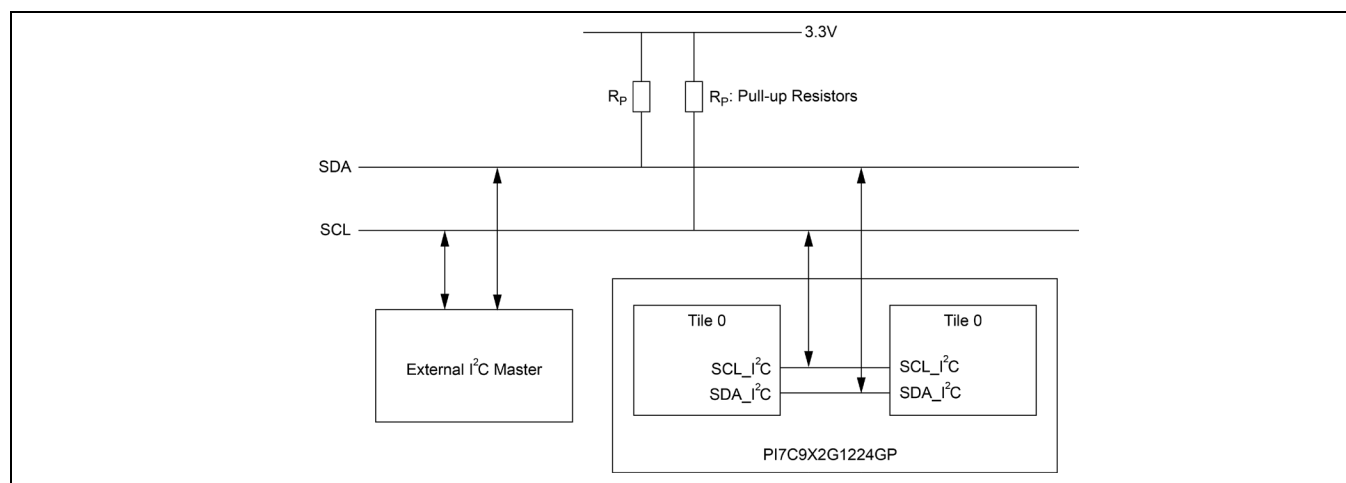
Figure 5-7 Standard Devices to I2C Bus Connection Block Diagram
