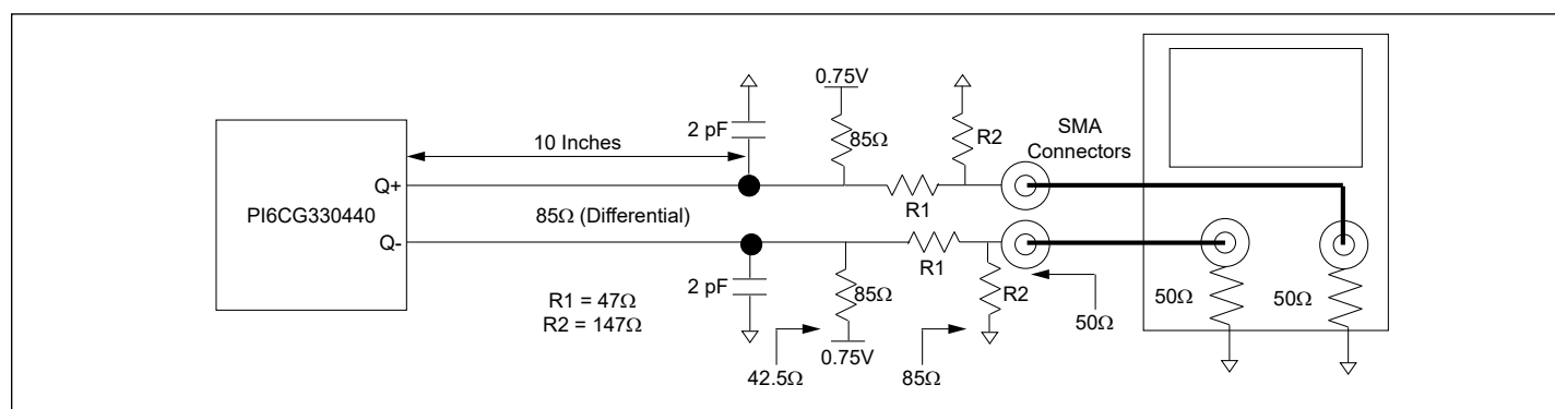
Figure 11. Test Setup for Double Termination
