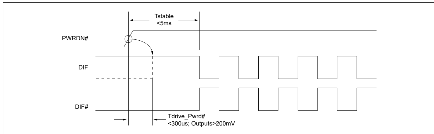
Figure 2. PWRGD Assertion Timing
