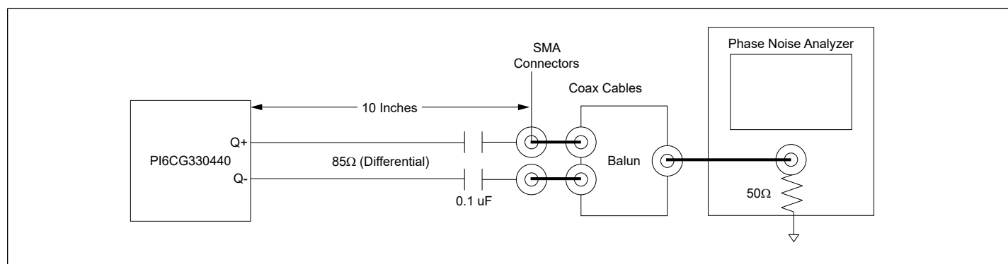
Figure 10. Test Setup for PCIe Jitter Measurement
