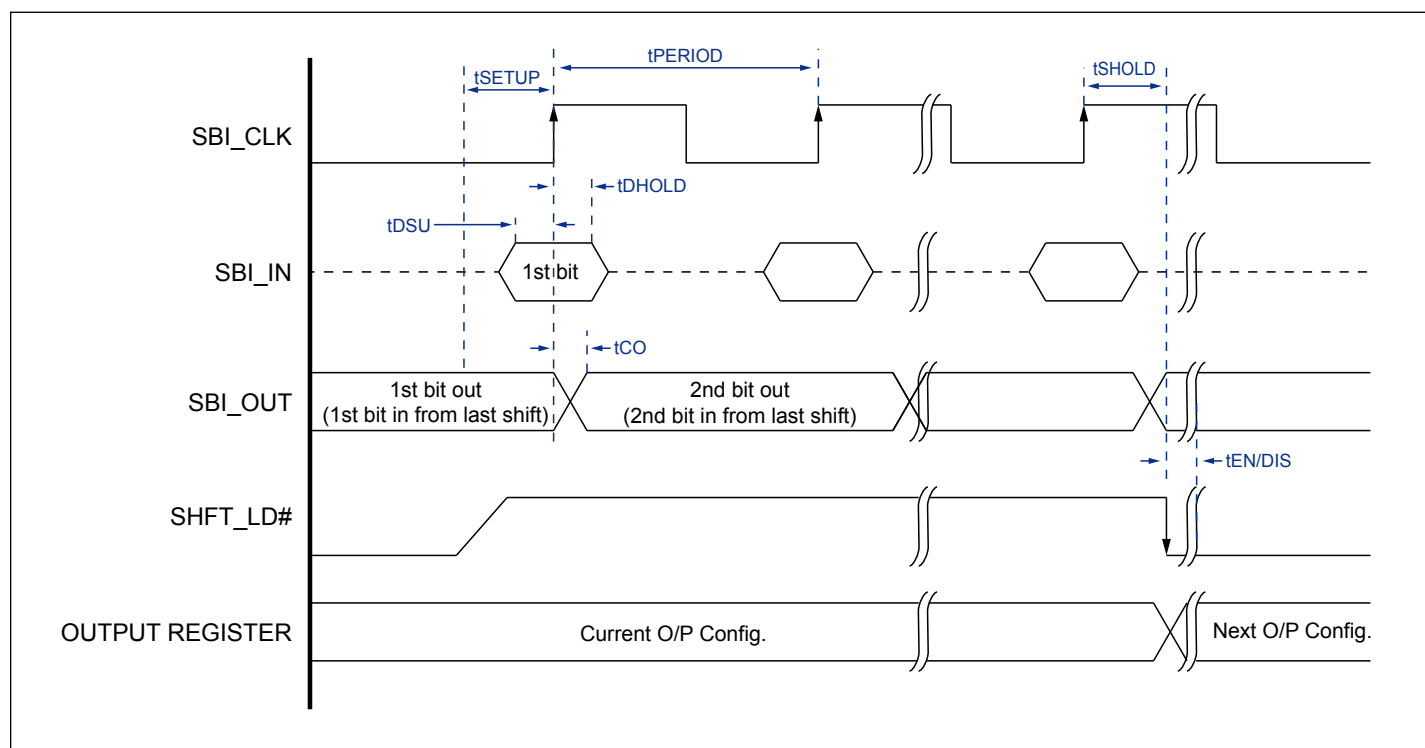
Figure 9. Side Band Interface Timing
