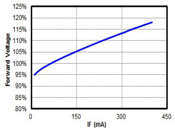
Forward Current vs. Forward Voltage ( T_j = 25^\circ\text{C} )
