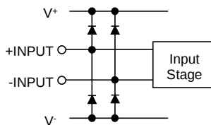
Figure 1. Simplified Schematic
