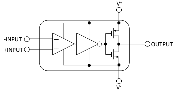
Push-Pull Output
