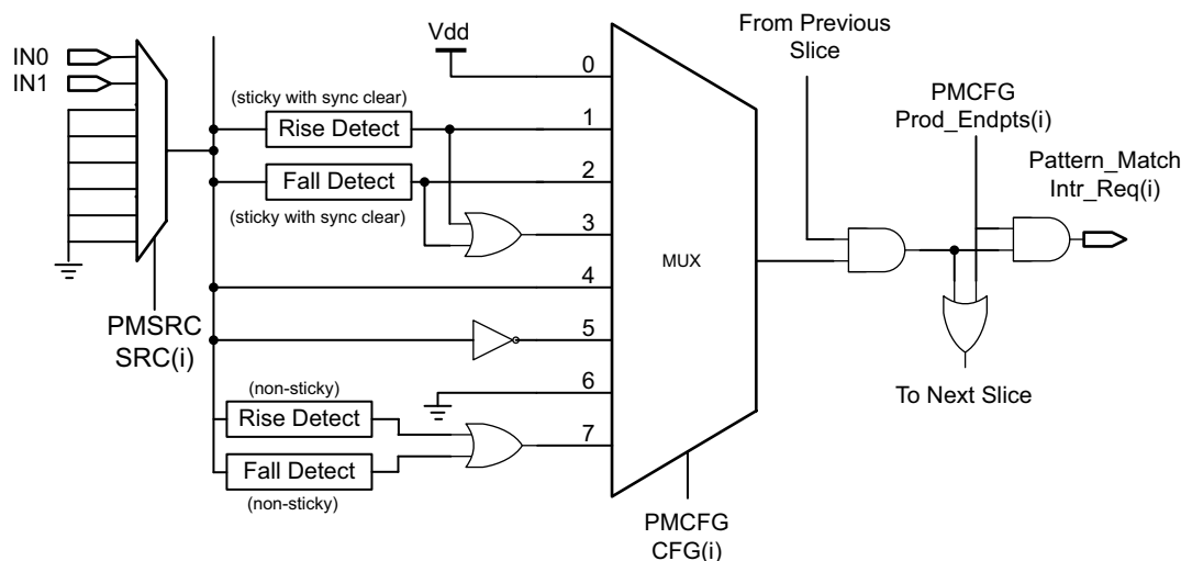
Fig 64. Secure pattern match bit slice with detect logic
