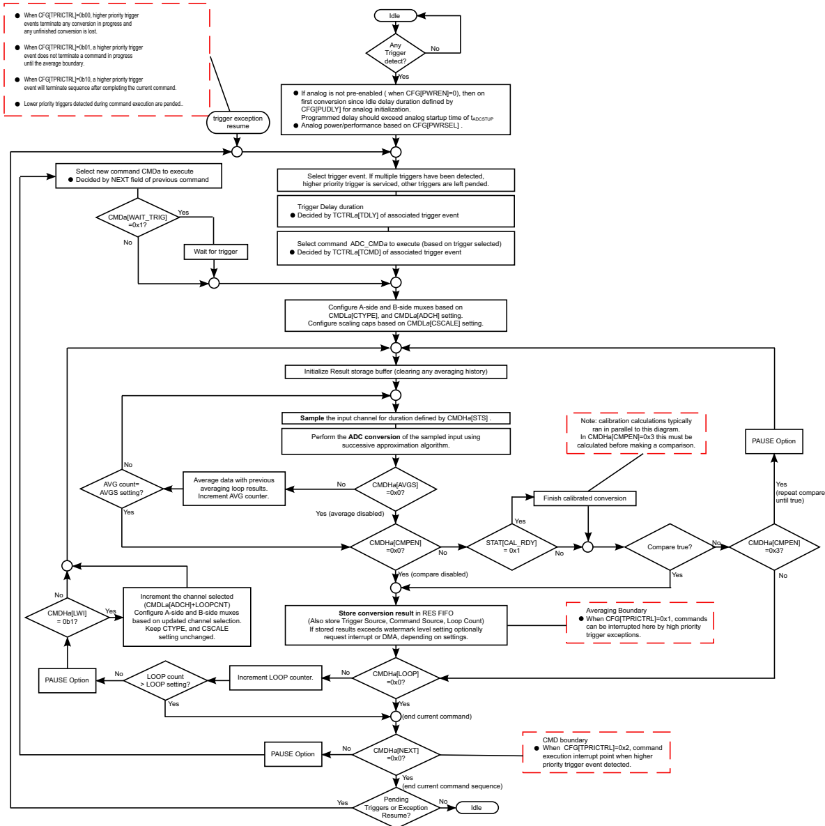
Fig 147. ADC command sequencing
