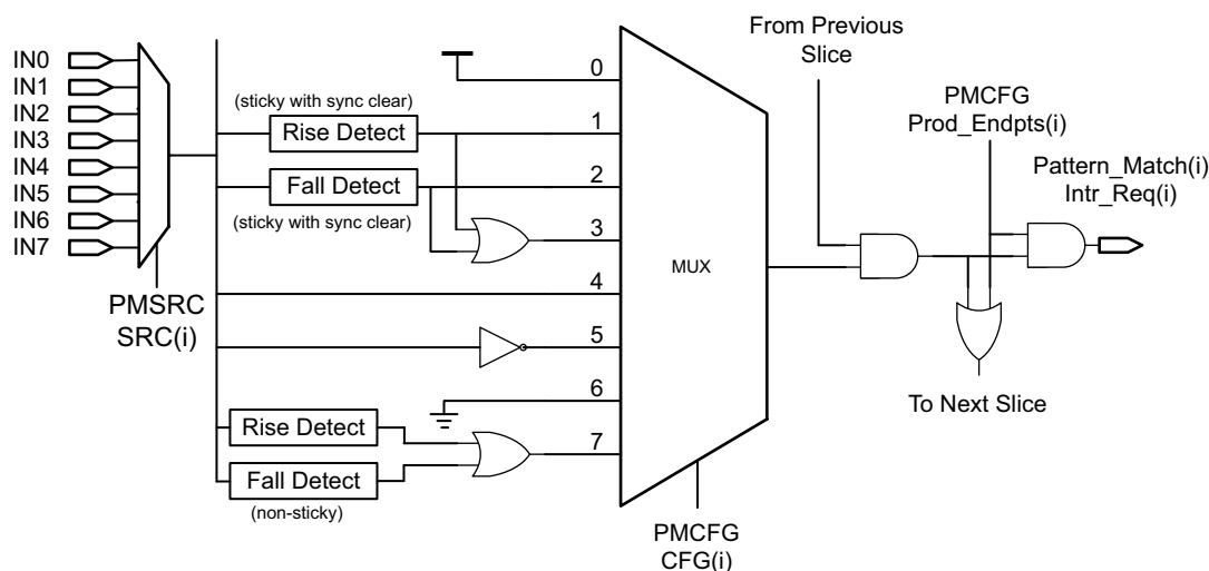
Fig 58. Pattern match bit slice with detect logic
