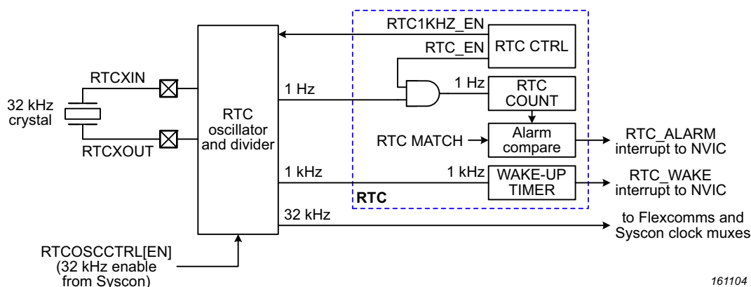
Fig 106. RTC clocking and block diagram
