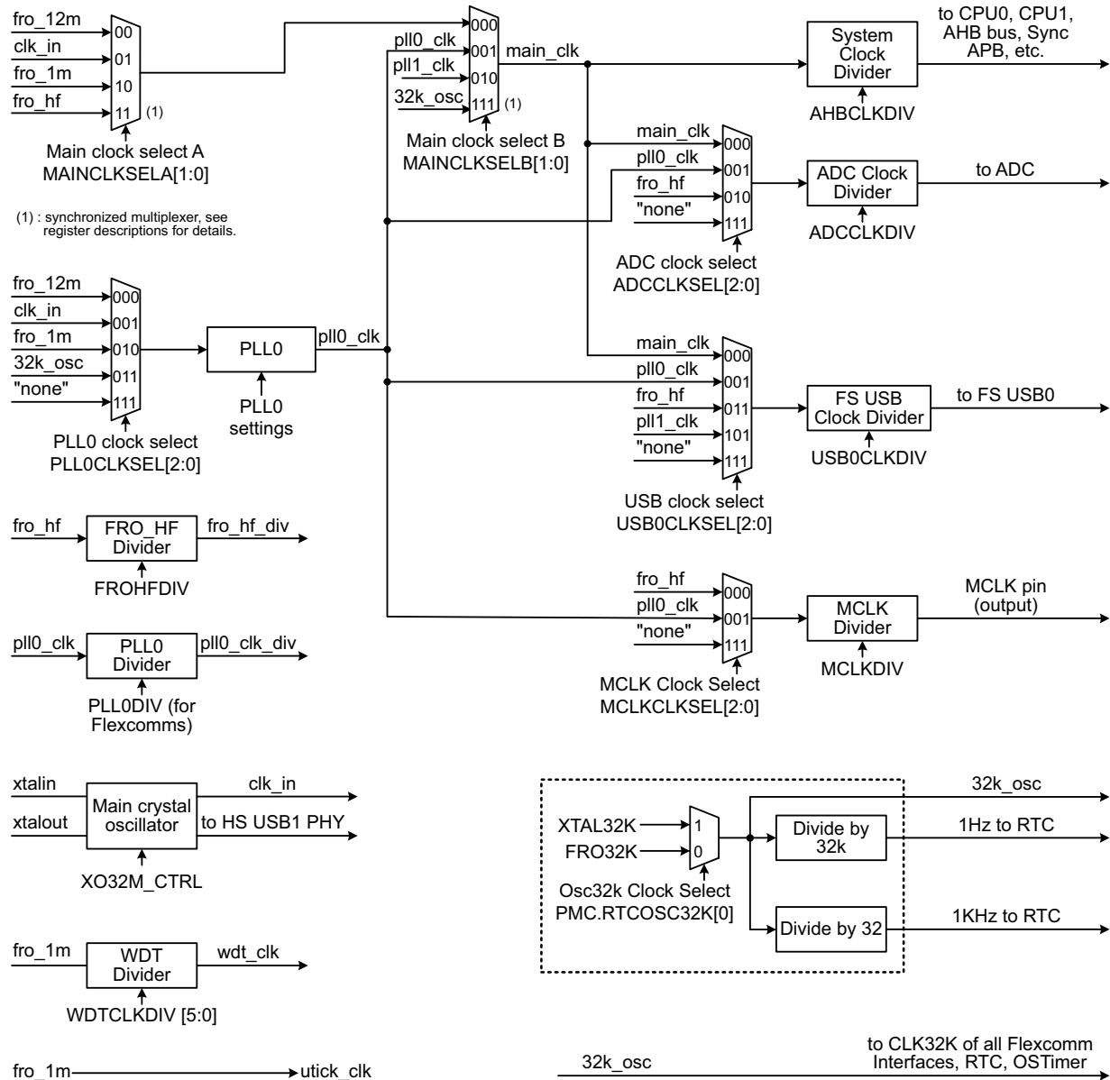
Fig 4. LPC55S6x Clock generation (Part 1 of 3)
