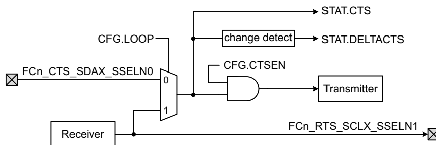
Fig 118. Hardware flow control using RTS and CTS
