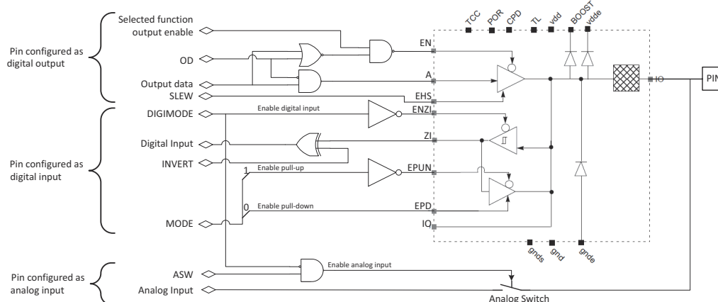
Fig 48. Standard GPIO pin configuration
