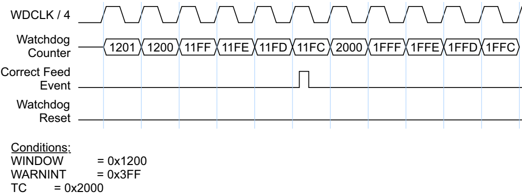
Fig 111. Correct watchdog feed with windowed mode enabled
