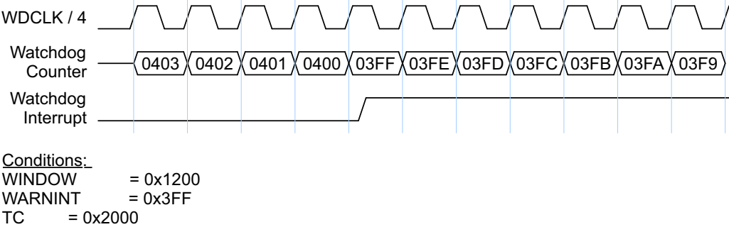
Fig 112. Watchdog warning interrupt
