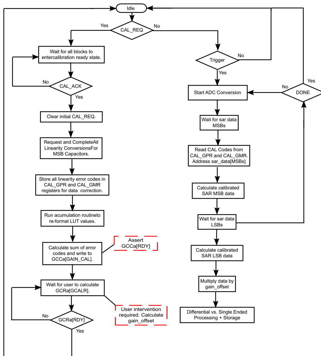
Fig 149. ADC calibration sequence
