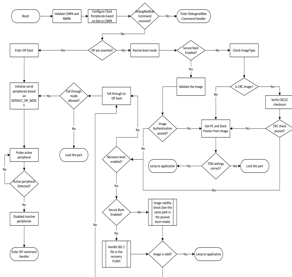
Fig 11. LPC55S6x/LPC55S2x/LPC552x boot flow chart for 1B
