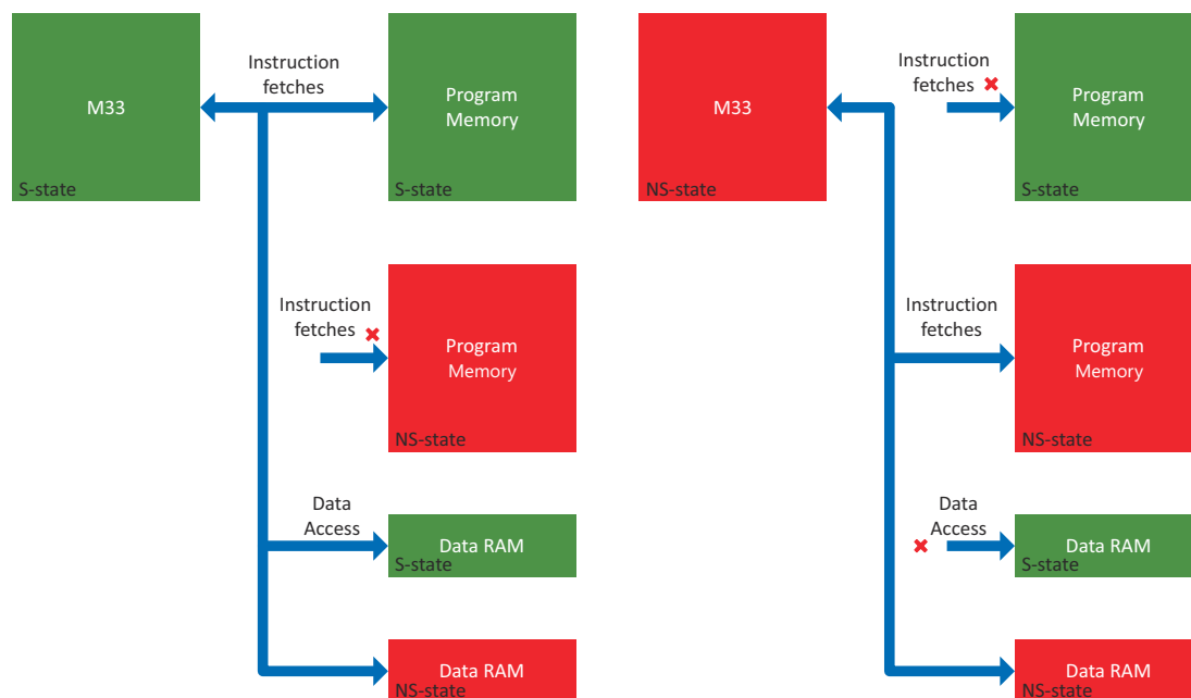
Fig 169. Secure state and Non-secure state view for TrustZone for ARMv8
