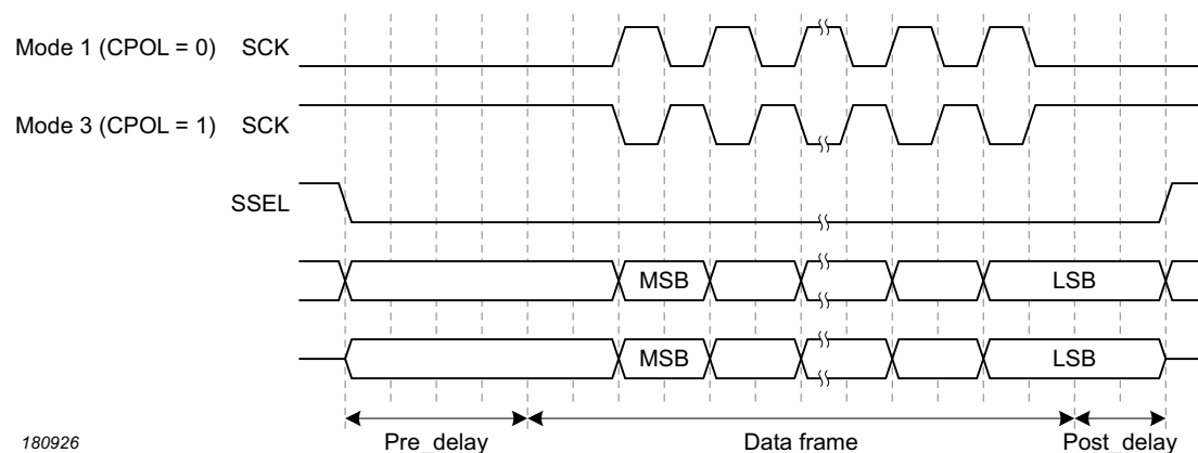
Fig 121. Pre_delay and Post_delay
