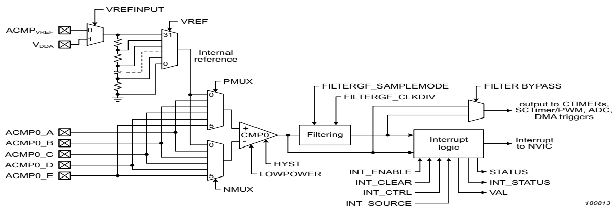
Fig 150. Comparator block diagram
