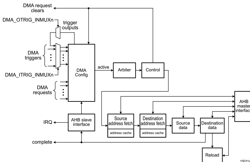
Fig 68. DMA block diagram
