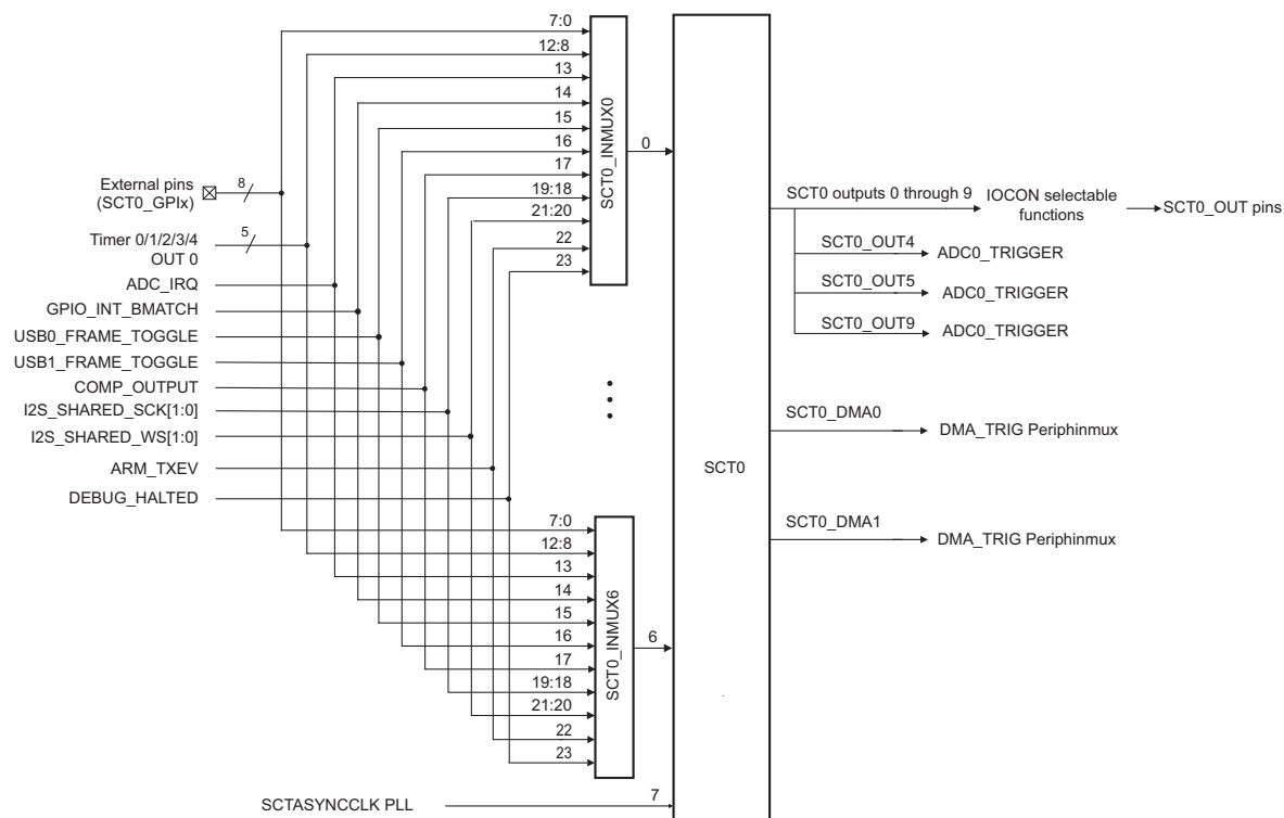
Fig 52. SCT0 input multiplexing
