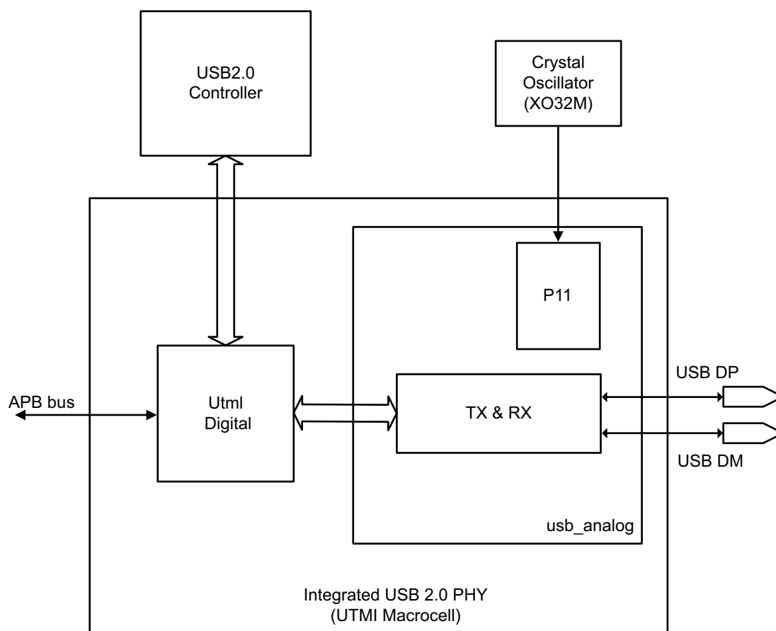
Fig 165. USB 2.0 PHY block diagram
