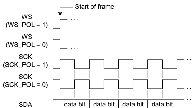
Fig 143. Data at the start of a frame, shown with both SCK and WS polarities
