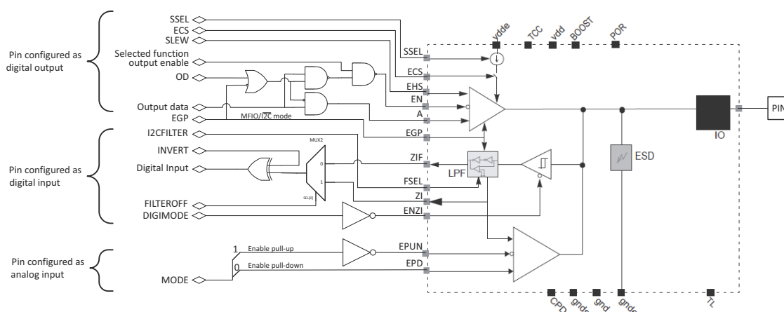
Fig 49. Combo I 2 C/GPIO pin configuration
