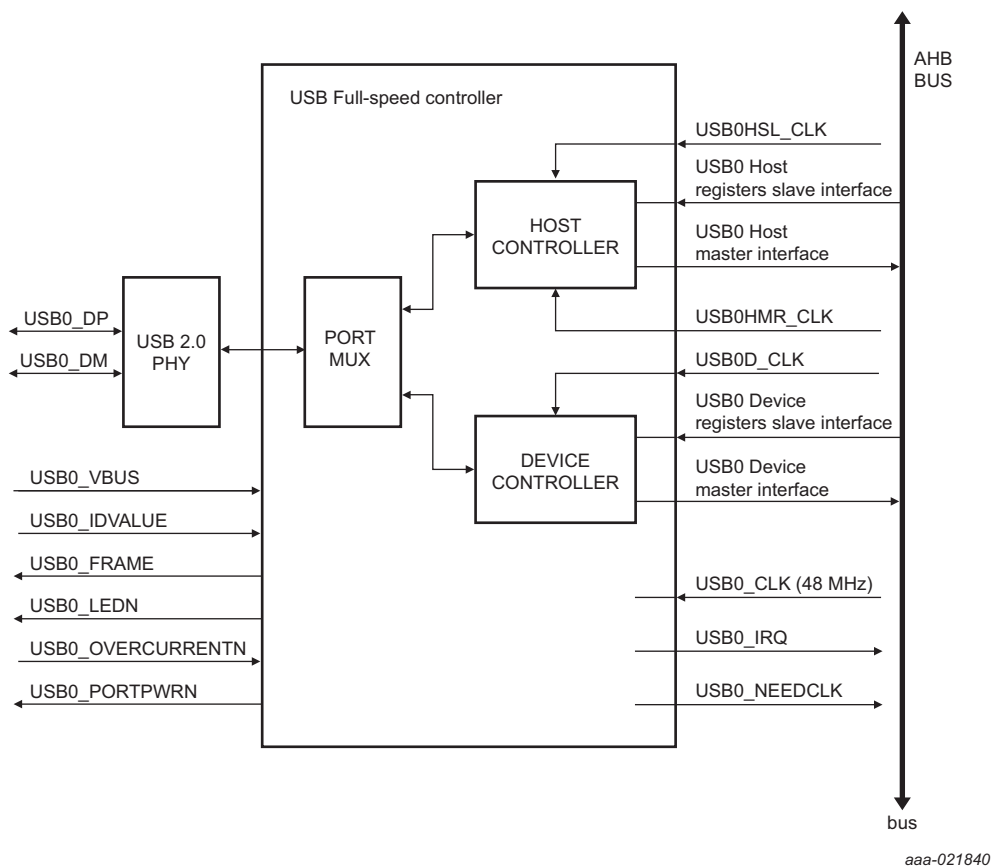
Fig 151. USB full-speed host/device controller block diagram
