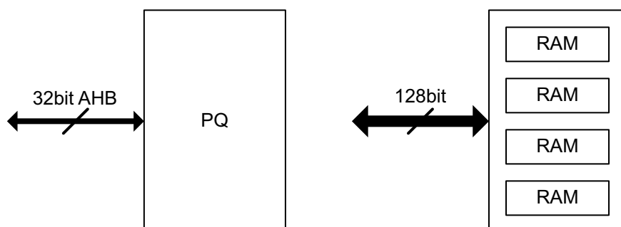
Fig 186. PowerQuad using RAM Bank 4 (16kB) as the 128bit Wide RAM scratch pad
