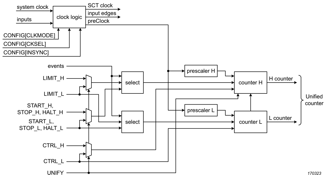
Fig 91. SCTimer/PWM counter and select logic
