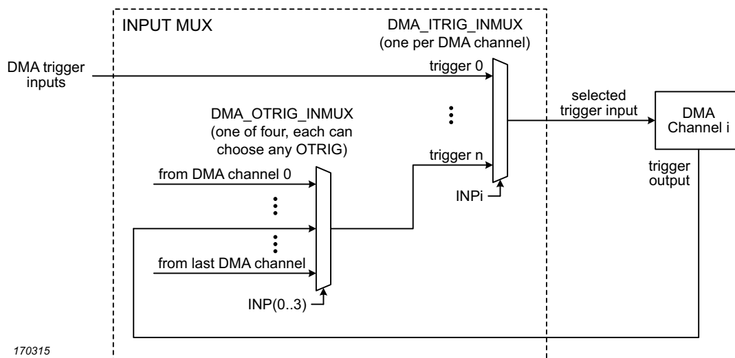
Fig 55. DMA trigger input multiplexing
