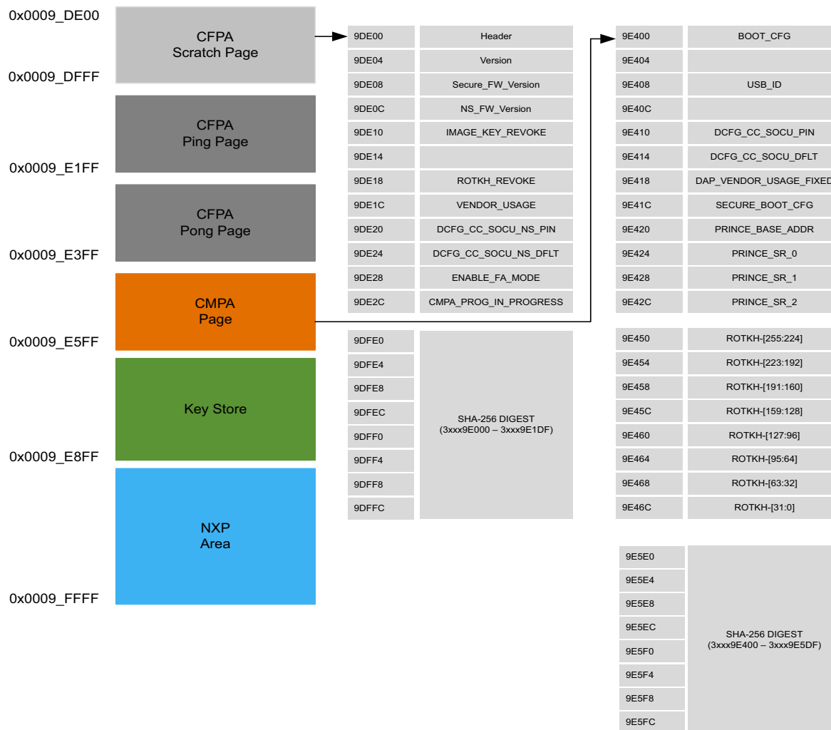
Fig 13. Protected Flash Region
