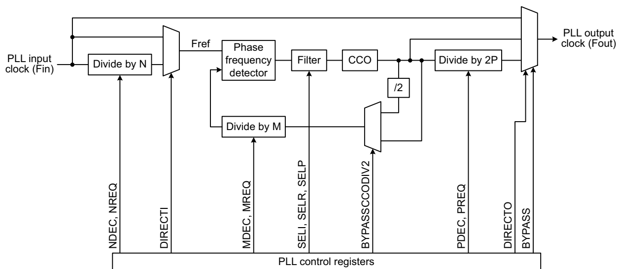
Fig 8. System PLL block diagram showing typical operation
