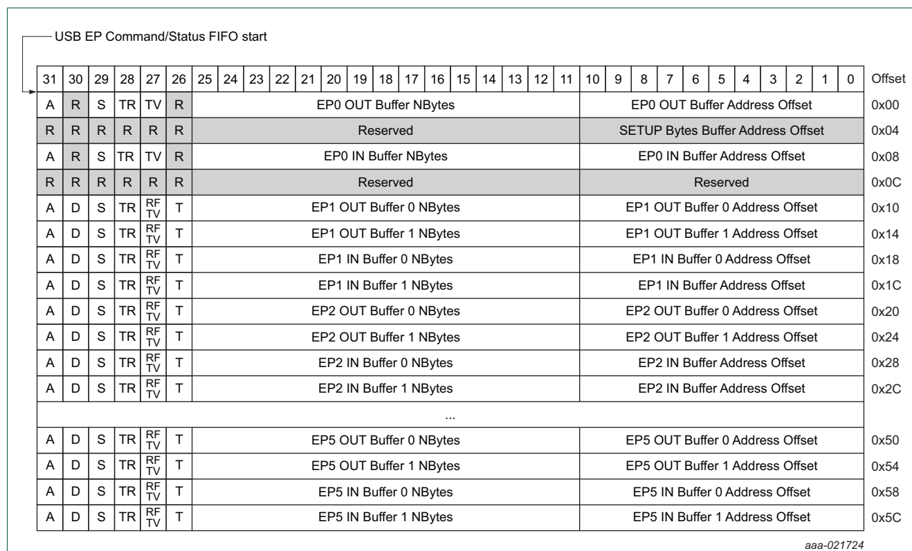
Fig 162. Endpoint command/status list (see also Table 829)
