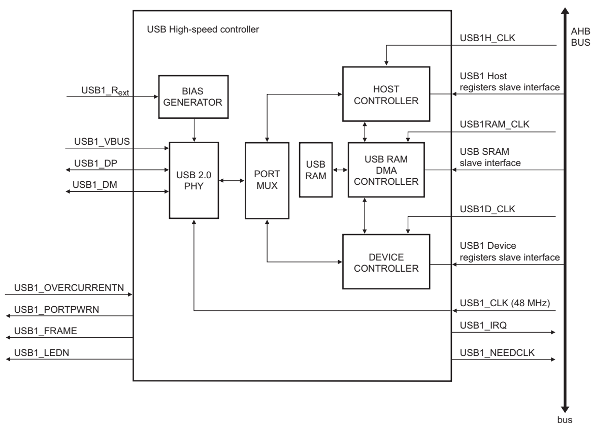
Fig 157. USB host controller block diagram
