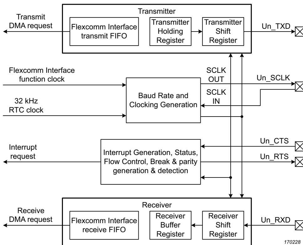
Fig 117. USART block diagram
