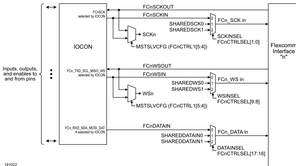
Fig 125. Shared signal connections for each Flexcomm Interface
