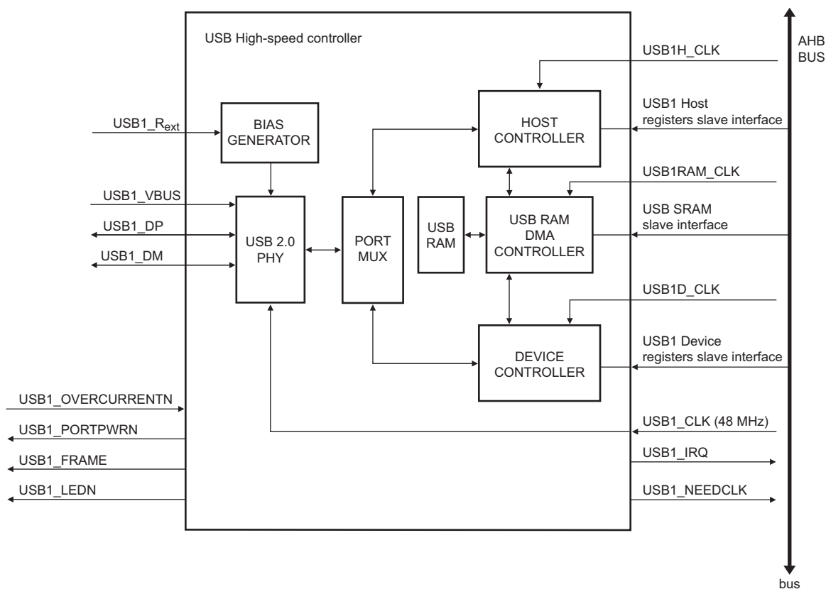
Fig 160. USB host/device controller block diagram
