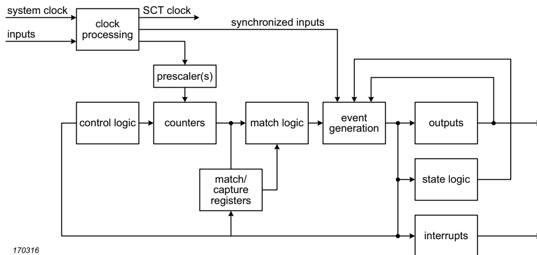
Fig 90. SCTimer/PWM block diagram
