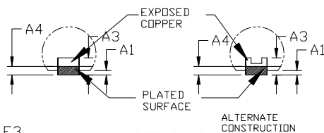
DETAIL B
