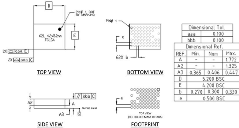
Figure 9: Package Drawing
