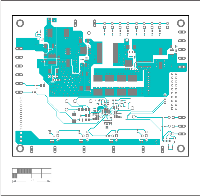
MAX25014 EV Kit PCB Layout—Top Layer
