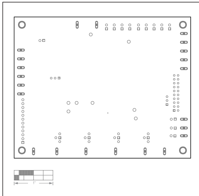
MAX25014 EV Kit PCB Layout—Bottom Silkscreen
