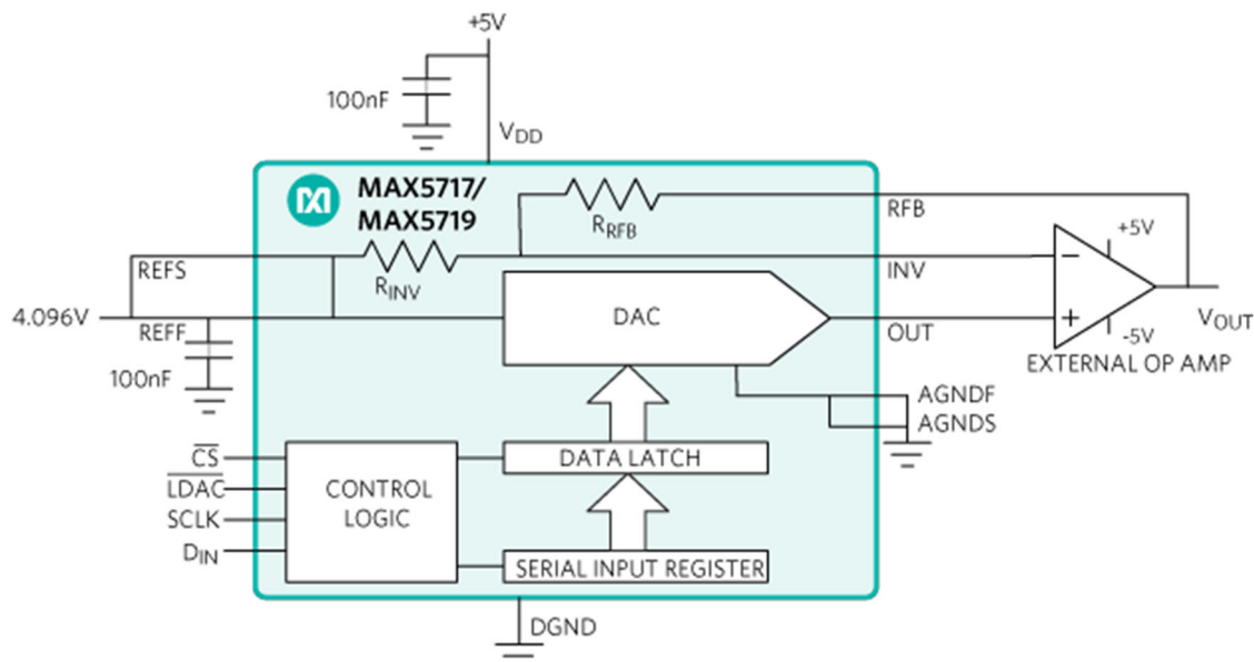
Figure 7. A block diagram of a 16-bit/20-bit DAC with a 3-wire SPI, QSPI™, MICROWIRE, and DSP-compatible serial interface.
