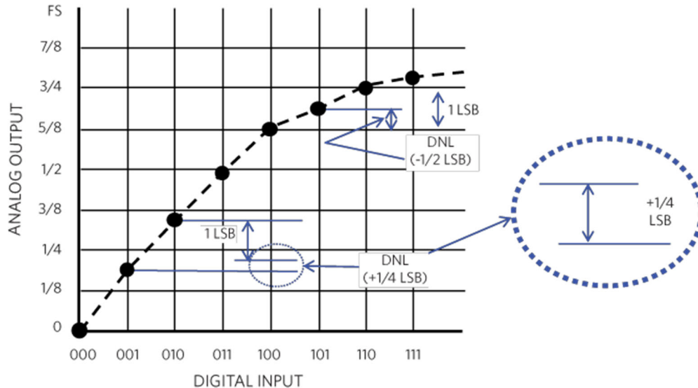
Figure 3. In this illustration, the DAC DNL determines the monotonicity of the converter, rendering this DAC to be a monotonic device.
