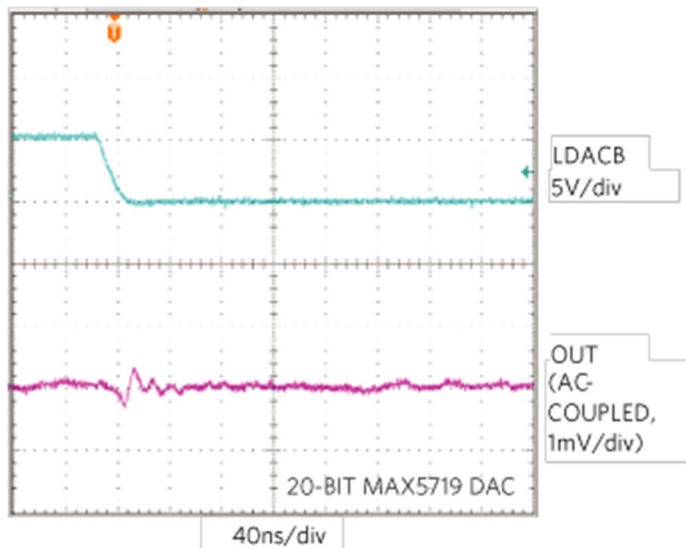
Figure 6. This R-2R DAC major carry (7FFF to 8000) output glitch is 0.05nV-s.
