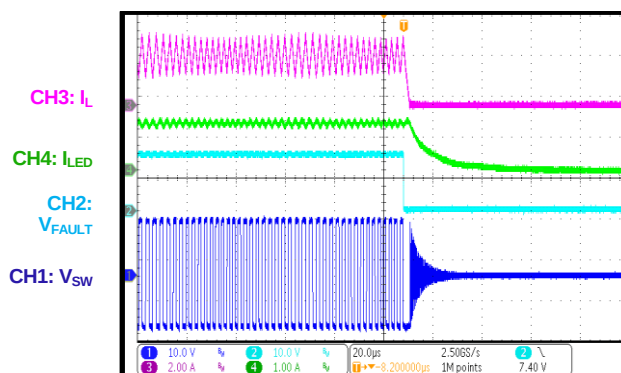
IREF Open Fault after IC Starts Up
