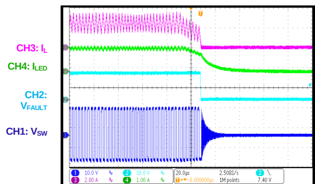
ISSET Open Fault after IC Starts Up
