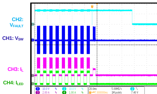
PWM Dimming LED+ short LED- entry
