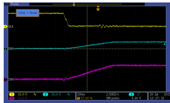
Figure 6: Switching with 100\Omega Resistance and Diode
