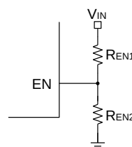
Figure 7: Enable Divider Circuit
