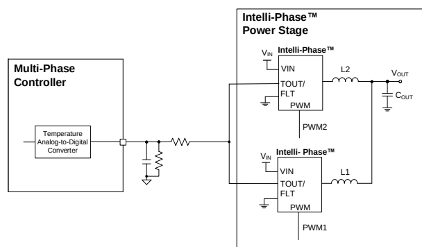
Figure 3: Multi-Phase Temperature Sense
