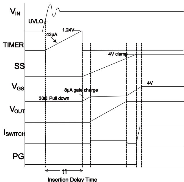
Figure 4: Start-Up Sequence
