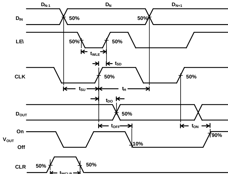
Figure 1: Timing Diagram
