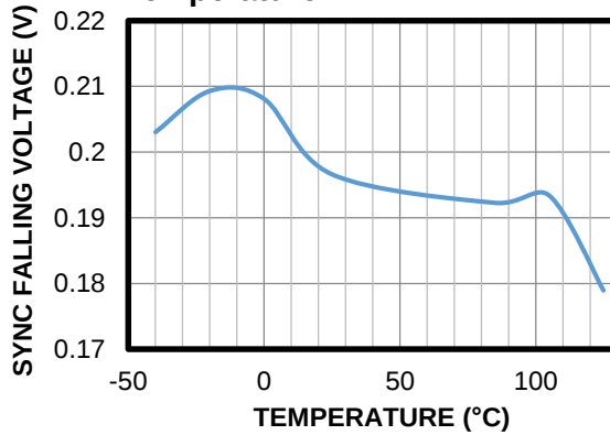
SYNC Falling Voltage vs. Temperature
