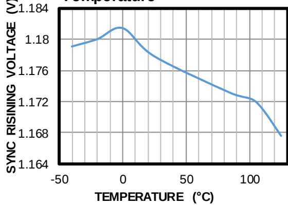
SYNC Rising Voltage vs. Temperature
