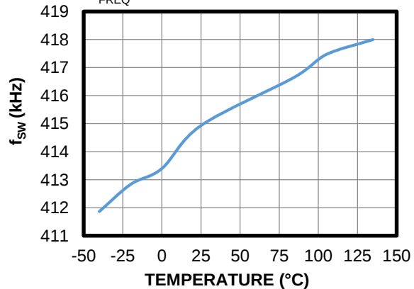
f_{SW} vs. Temperature R_{FREQ} = 86.6k\Omega
