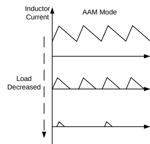
Figure 5: AAM Mode
