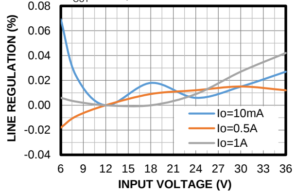
Line Regulation
