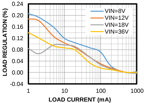
Load Regulation
