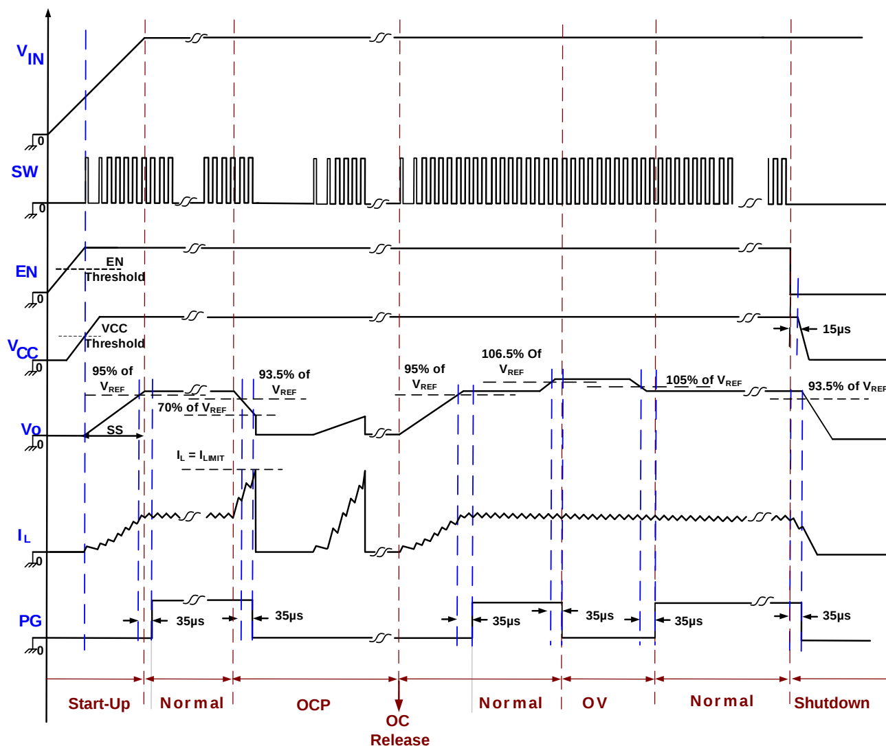
Figure 2: Timing Sequence
