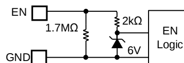
Figure 2: Zener Diode between EN and GND
