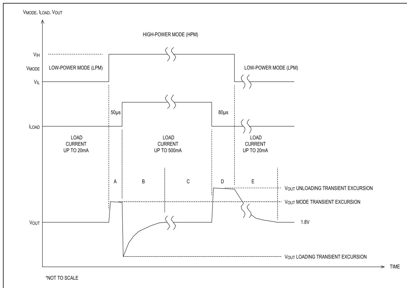
Figure 1. MODE Transition
