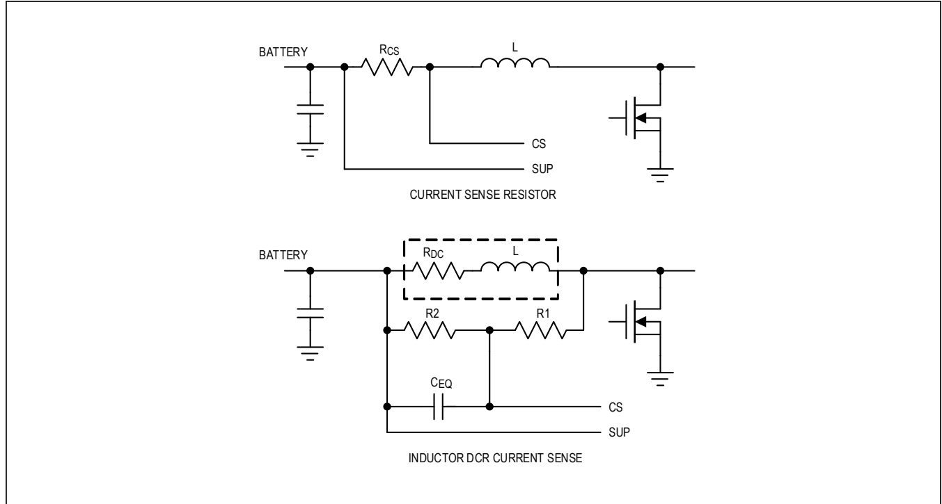
Figure 1. Current-Sense Configurations
