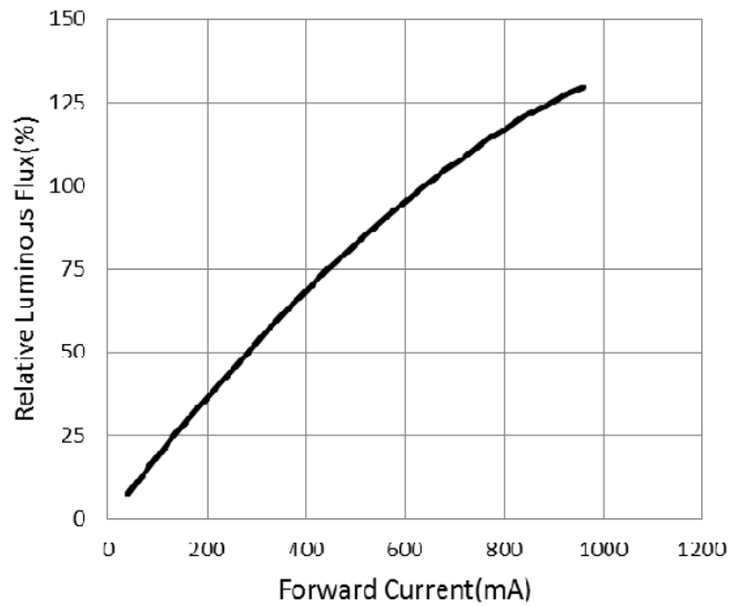
I_f ----- Relative Luminous flux
