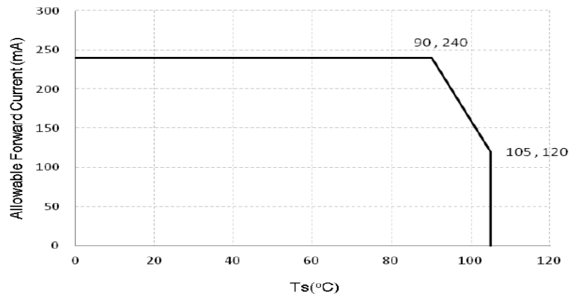
Allowable Forward Current vs. Case Temperture ( T_j<120^\circ\text{C} )
