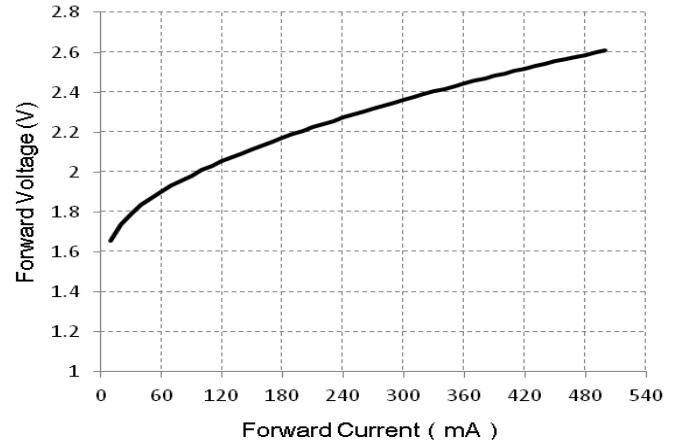
Forward Current vs. Forward Voltage ( T_j=25^\circ\text{C} )
