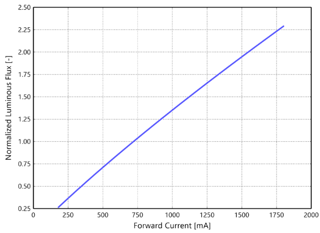
Figure 3g. Typical normalized light output vs. forward current for L2C6-xxxxxL08C1500 at T_j = 85^\circ\text{C} .
