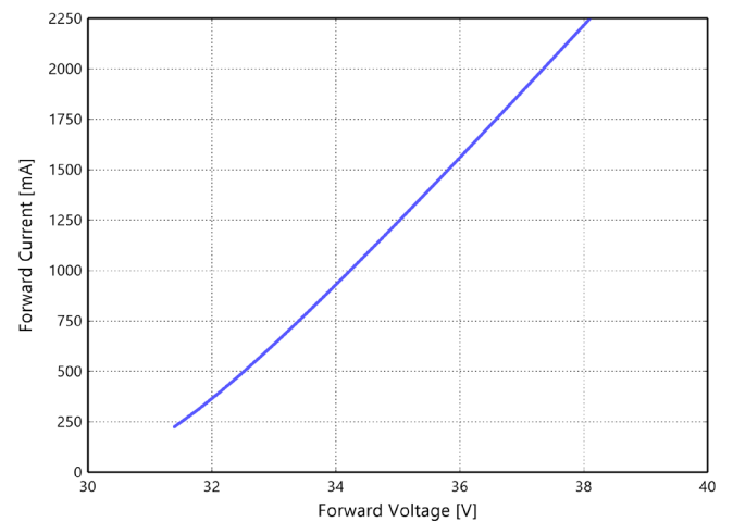
Figure 4h. Typical forward current vs. forward voltage for L2C6-xxxxxL10C1500 at T_j=85^{\circ}\text{C} .
