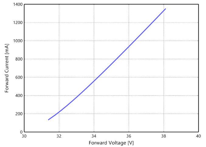
Figure 4f. Typical forward current vs. forward voltage for L2C6-xxxxxL06C1500 at T_j=85^{\circ}\text{C} .
