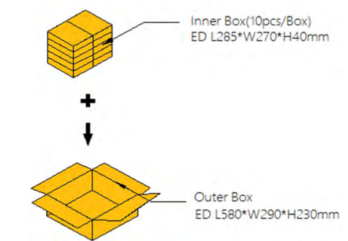
Figure 12. Dimensions for outer box packaging for LUXEON CS CoB.
