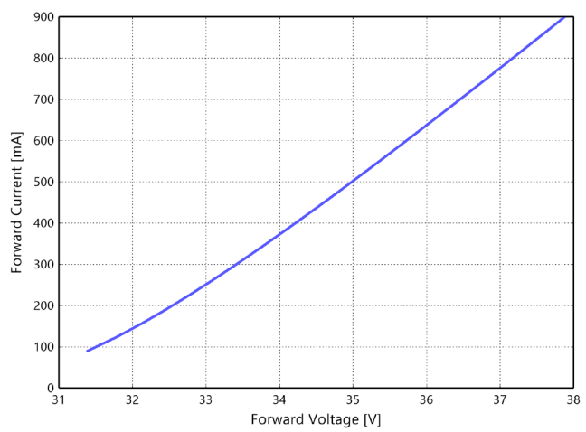
Figure 4d. Typical forward current vs. forward voltage for L2C6-xxxxxL04C0900 at T_j=85^{\circ}\text{C} .
