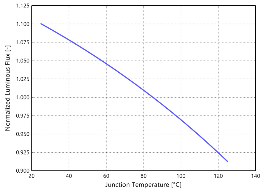
Figure 2. Typical normalized light output vs. junction temperature for L2C6-xxxxxLxxCxx00 at specified test current.
