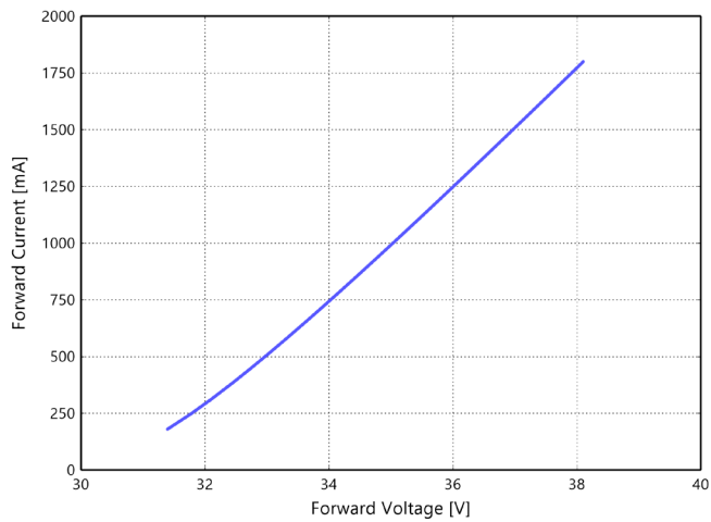
Figure 4g. Typical forward current vs. forward voltage for L2C6-xxxxxL08C1500 at T_j=85^{\circ}\text{C} .
