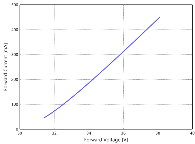
Figure 4b. Typical forward current vs. forward voltage for L2C6-xxxxxL02C0900 at T_j=85^{\circ}\text{C} .
