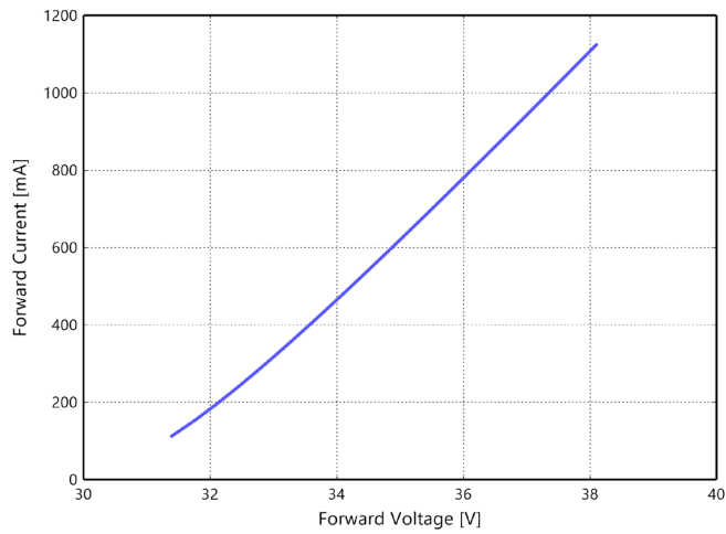
Figure 4e. Typical forward current vs. forward voltage for L2C6-xxxxxL05C1300 at T_j=85^{\circ}\text{C} .
