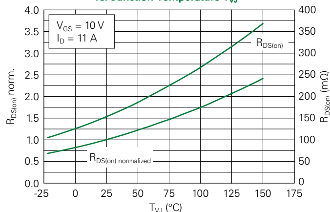
Fig. 5. Drain-Source On-state Resistance R_{DS(on)} vs. Junction Temperature T_{VJ}
