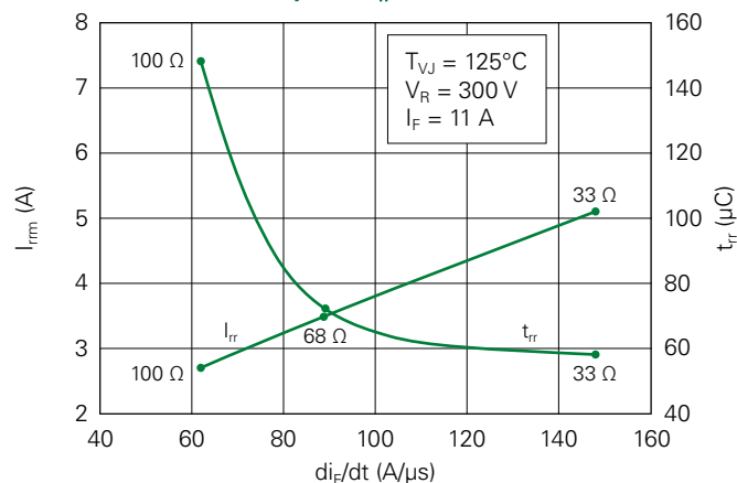
Fig. 21. Reverse Recovery Current I_{rrm} and Reverse Recovery Time t_{rr} vs. Commutation di_F/dt
