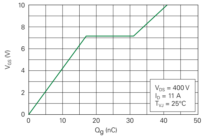
Fig. 8. Typical Gate Charge
