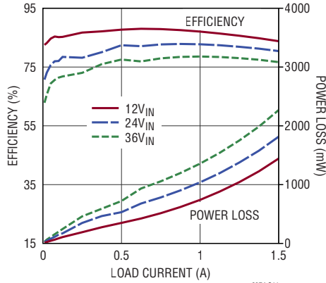
Efficiency and Power Loss, V_{OUT} = 5V , f_{SW} = 2MHz
