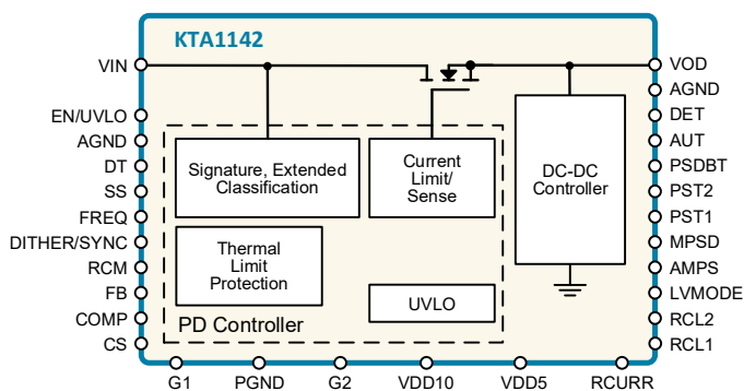
72W/90W (802.3bt-Compliant) PoE PD and DC-DC Controller
