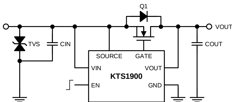
Figure 4. Typical Application
