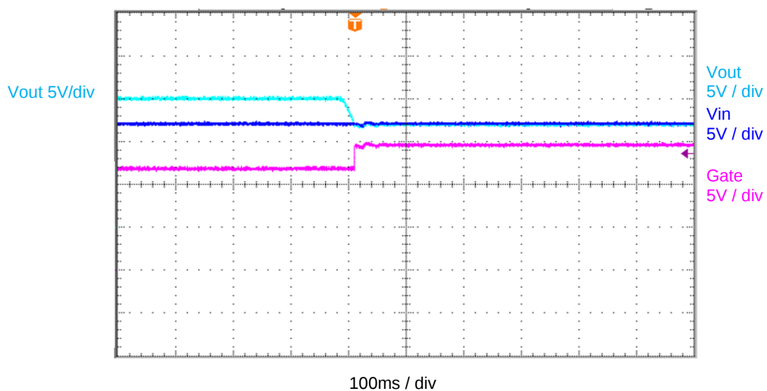
Figure 12. OR-Ing Performance VINB = 15V Cut out When VINA = 12V
