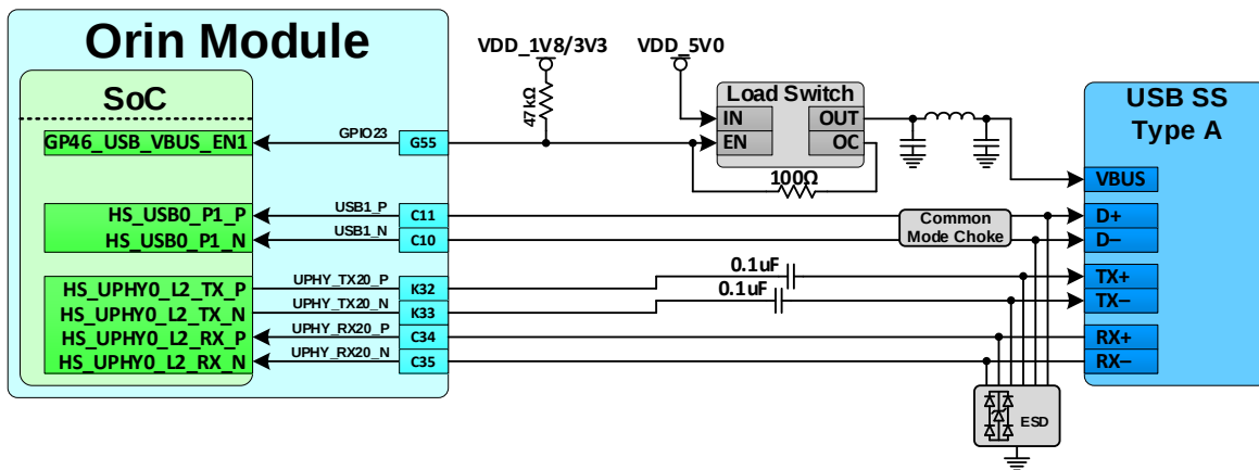
Figure 7-1. Simple USB Type A Connection Example
