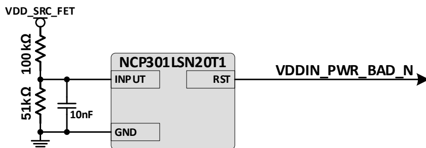
Figure 5-12. VIN Loss Detection Circuit
