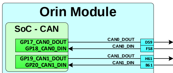
Figure 16-1. Orin Module CAN Connections
