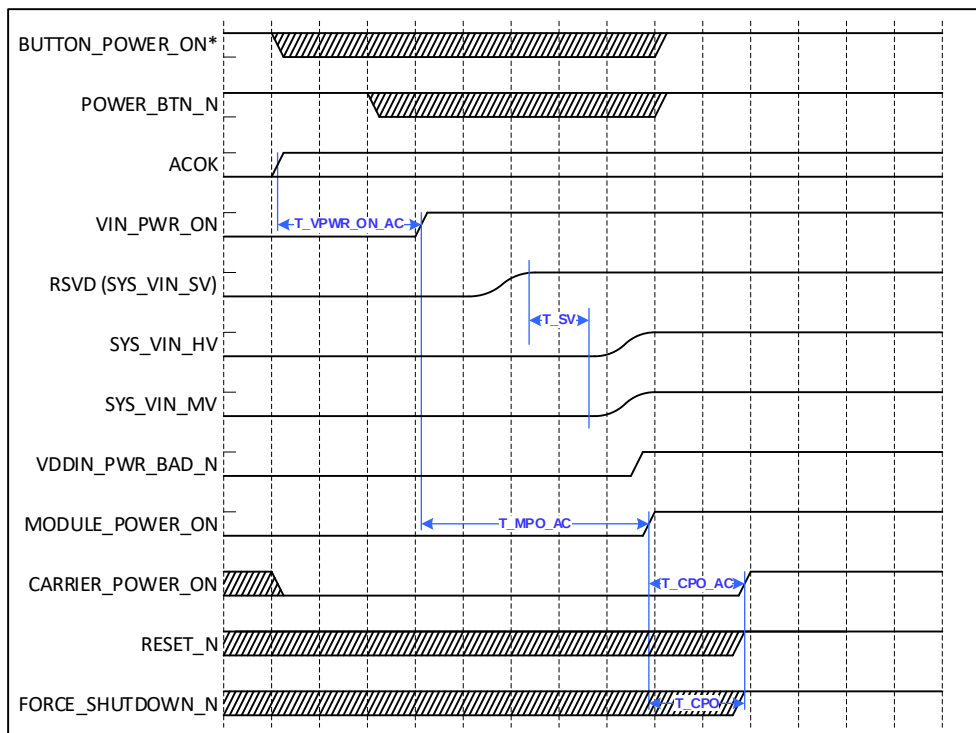
Figure 5-9. Power-OFF to On Sequence Auto Power-On Case
