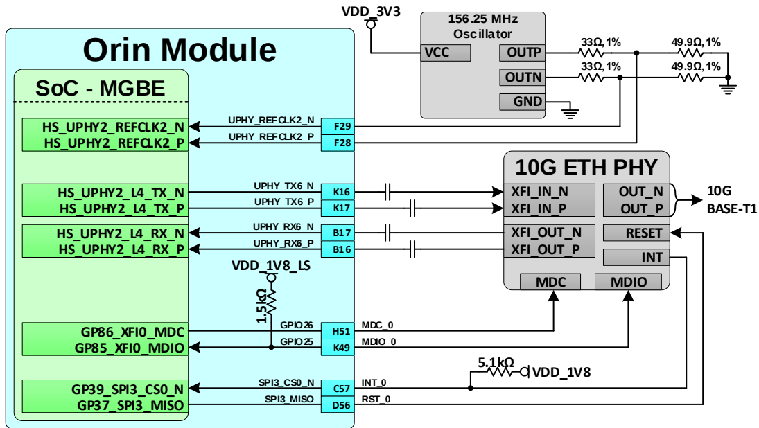
Figure 7-8. MGBE Connection Example – 10G Ethernet PHY
