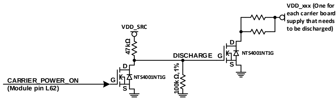
Figure 5-11. Power Discharge
