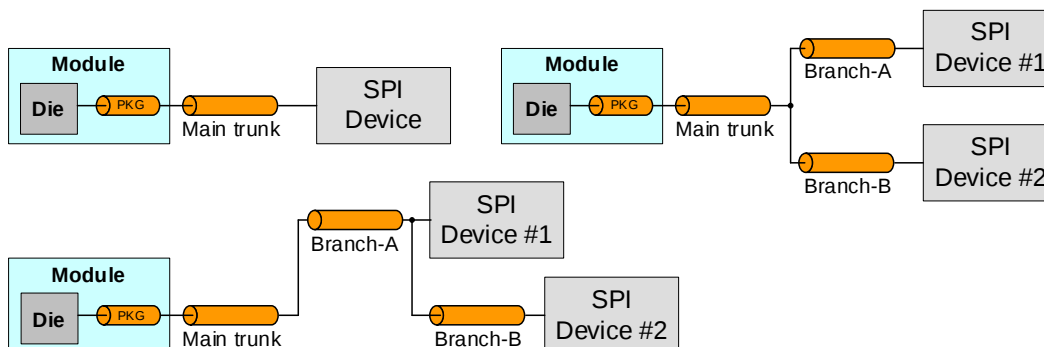
Figure 14-3. SPI Topologies
