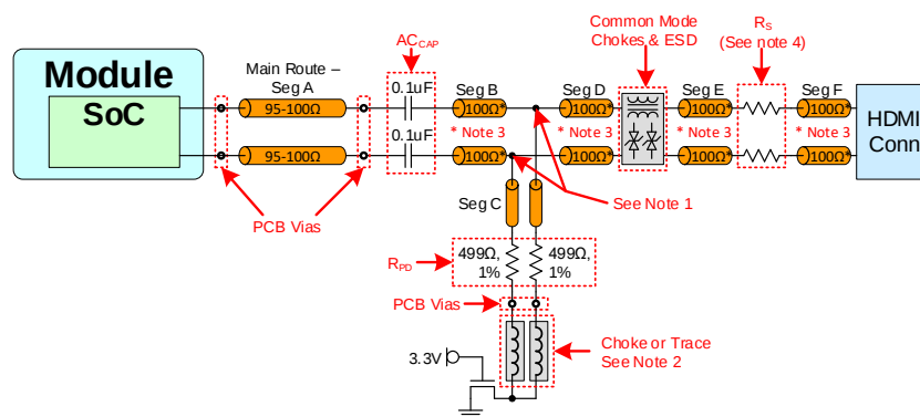
Figure 9-5. HDMI CLK and Data Topology
