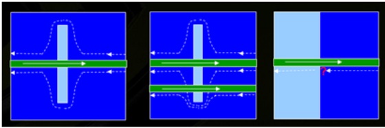
Figure 26-6. Power Plane Cuts Example
