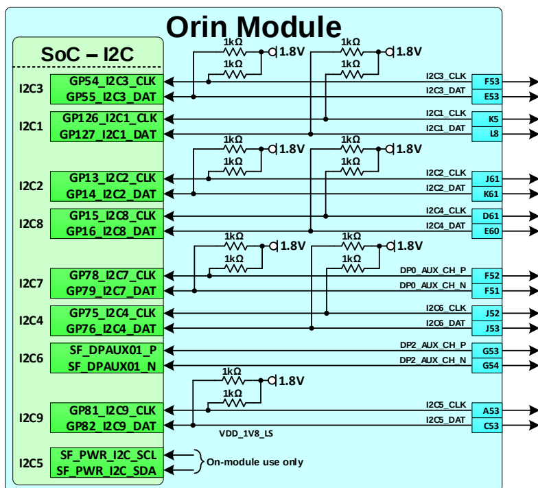
Figure 13-1. I2C Connections
