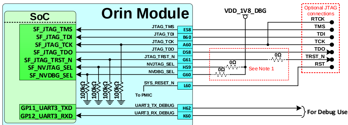
Figure 18-1. JTAG and UART Debug Connections
