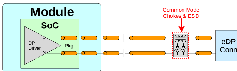
Figure 9-3. DP and eDP Differential Main Link Topology
