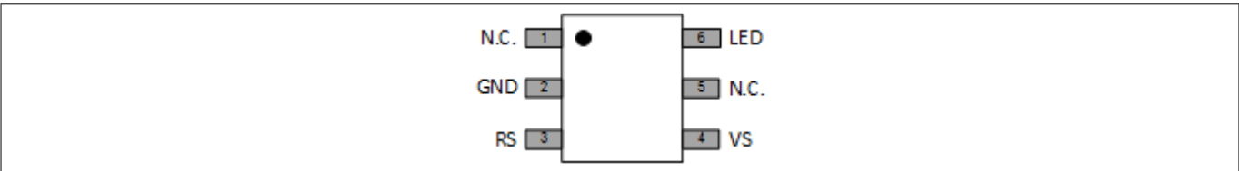
Figure 2 Pinout BCR431U
