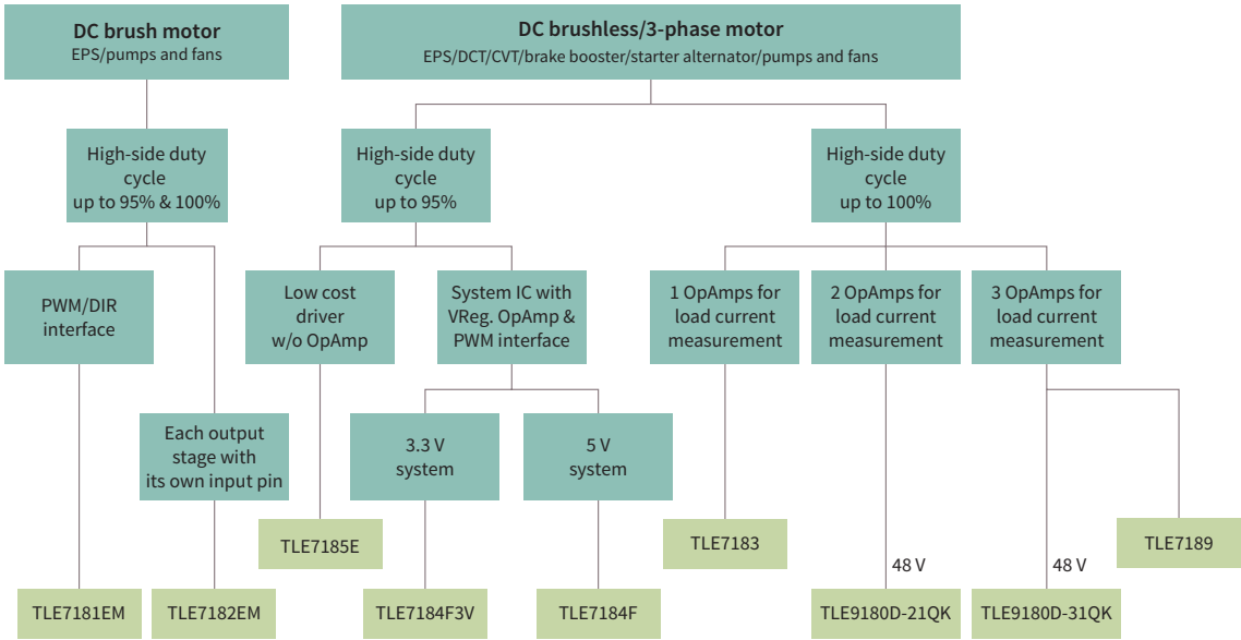
Image 14: Selection tree gate drivers ICs
