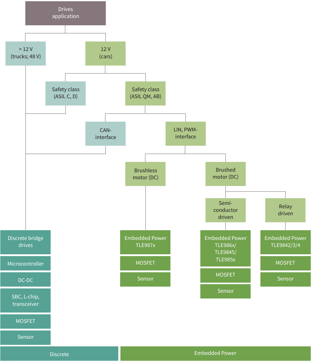
Image 6: The decision tree helps you to find the best fit: An Embedded Power-device or a less integrated solution.
