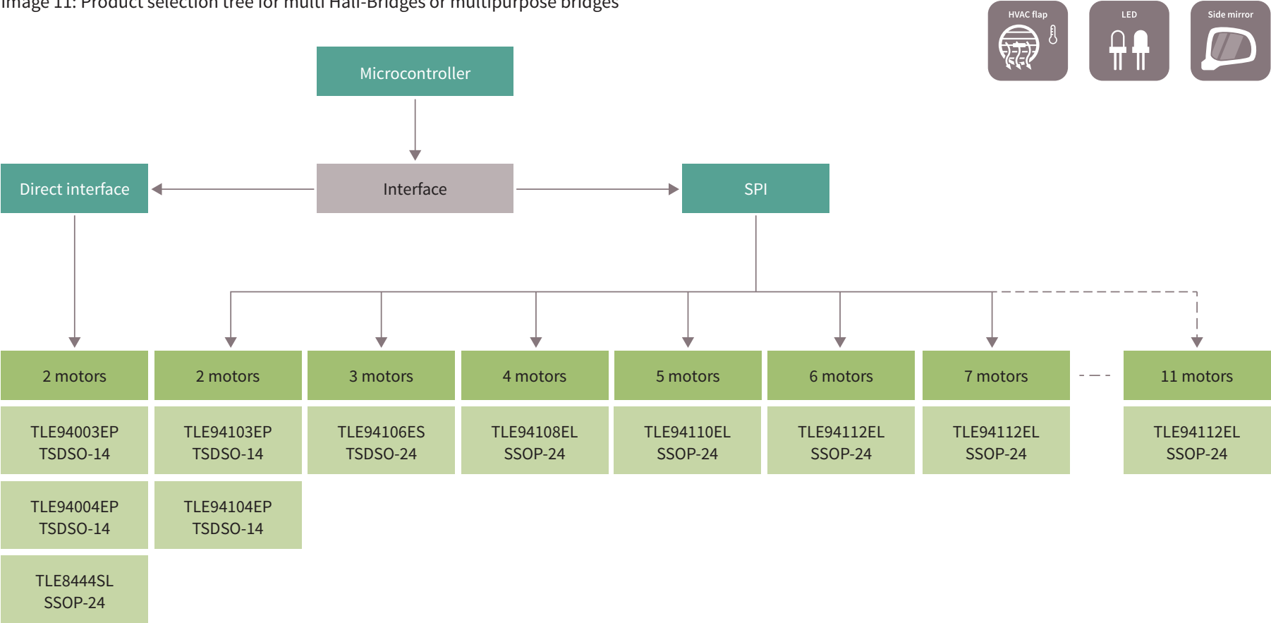
Image 11: Product selection tree for multi Half-Bridges or multipurpose bridges
