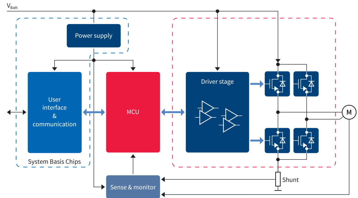
Image 10: Block diagram of DC motor control using components for medium integration
