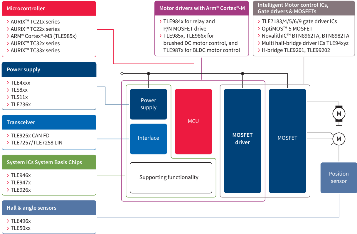
Image 4: Components from Infineon cover each function of the application
