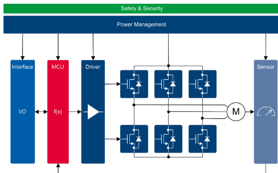
Image 13: Simplified block diagram of a 3-phase motor drive using discrete components
