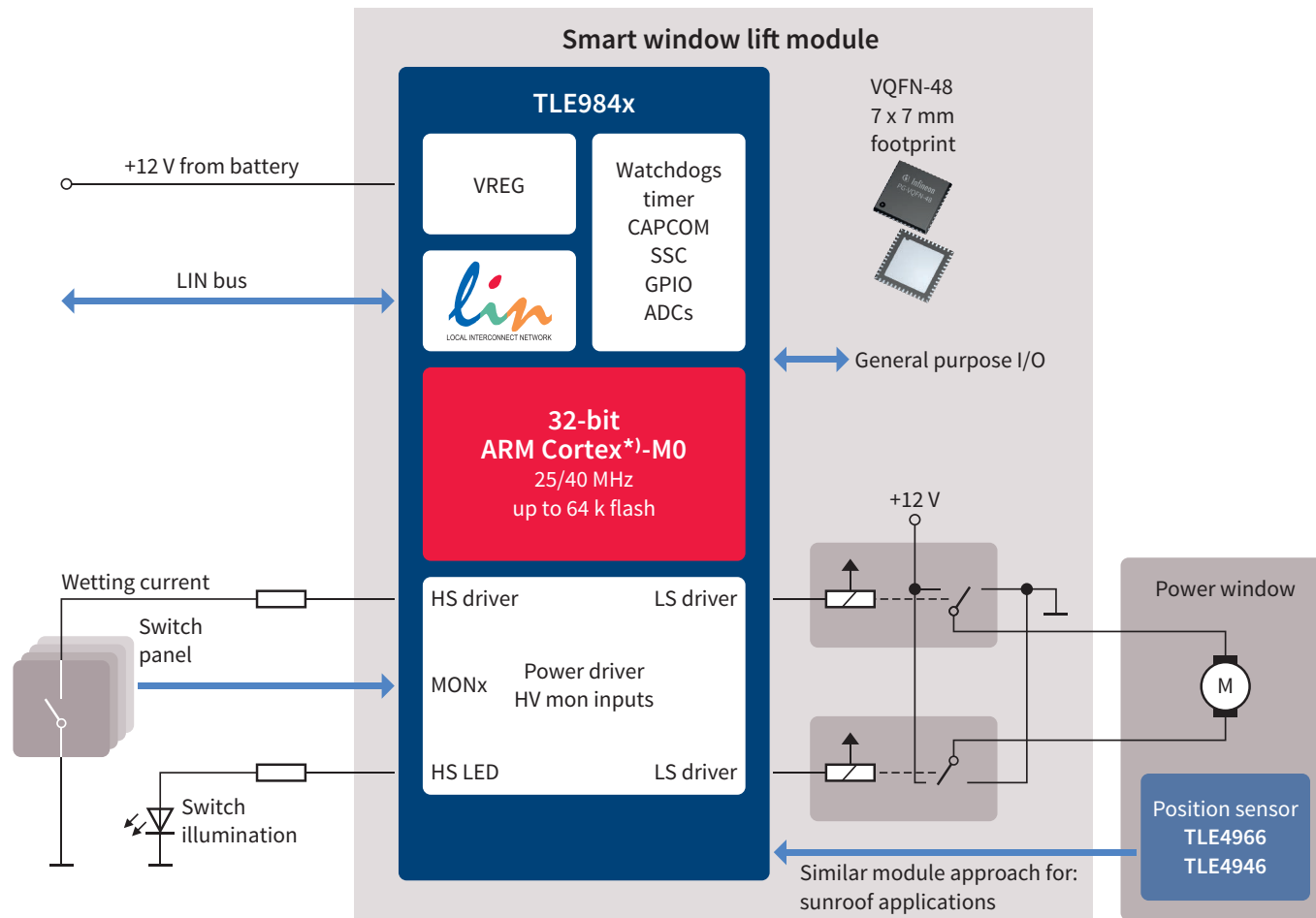
Image 7: Embedded Power ICs TLE984xQX: smart window lift application diagram
