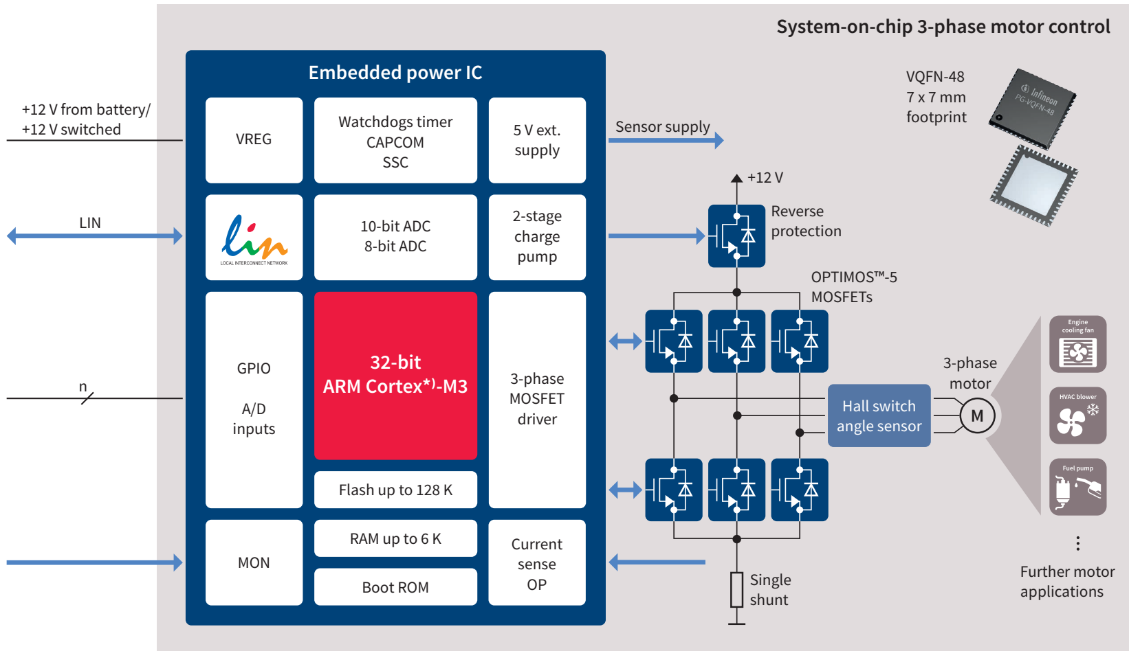
Image 8: TLE987x Infineon Embedded Power IC: 3-phase motor driver with integrated ARM® Cortex™-M3 MCU
