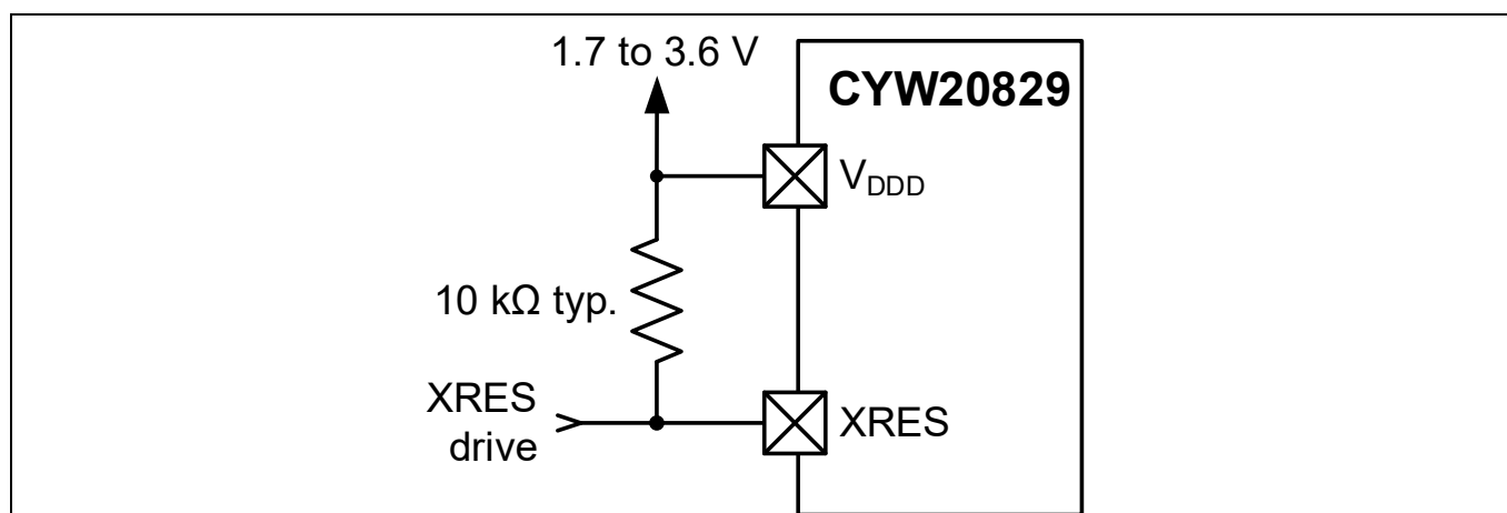
Figure 5 XRES connection diagram
