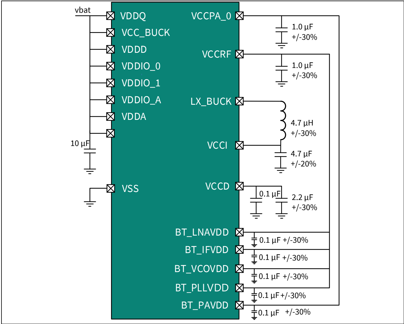
Figure 7 CYW20829 power topology
