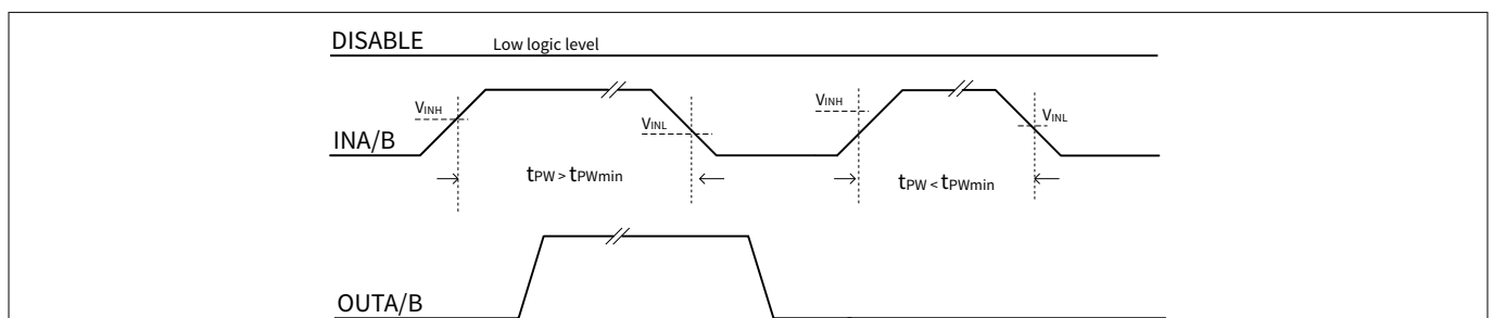
Figure 11 Minimum pulse that changes the output state
