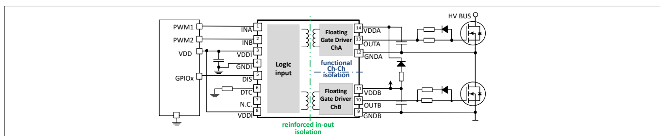
Figure 1 Application diagram
