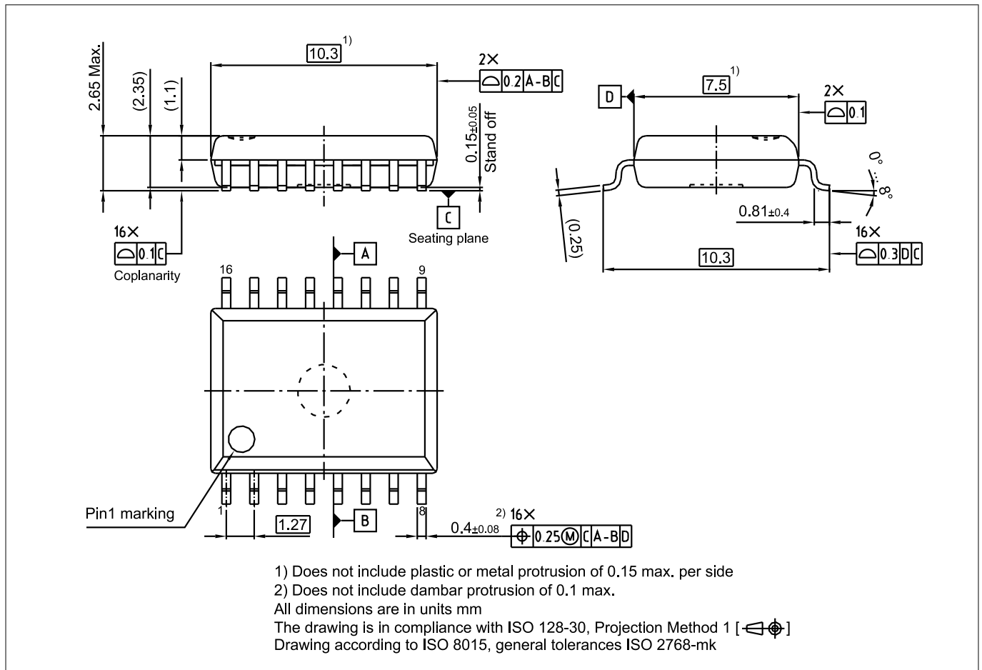
Figure 21 DSO16-300mil outline
