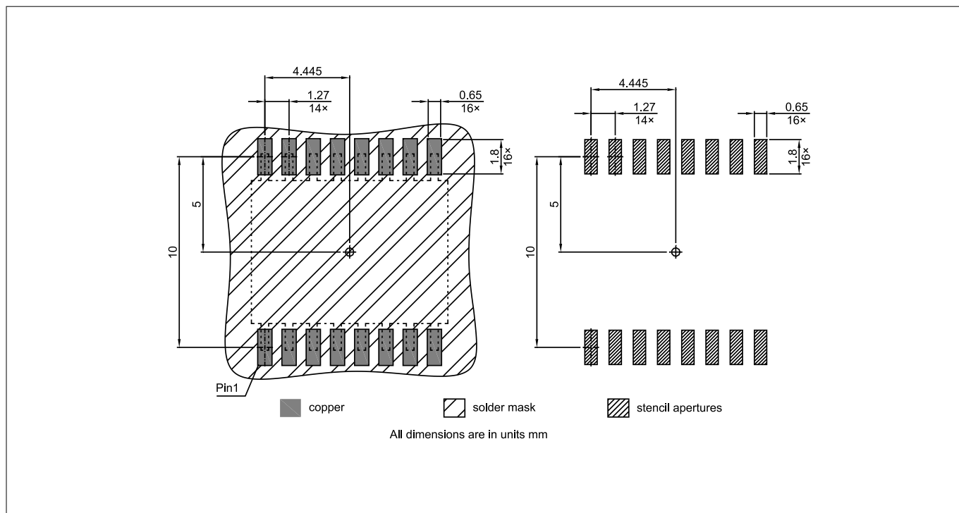
Figure 22 DSO16-300mil footprint
