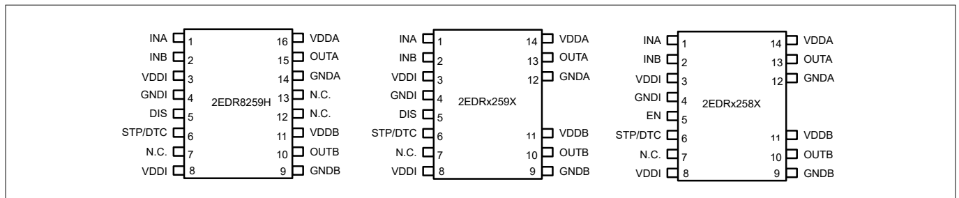
Figure 2 Pin configuration (top side view)
