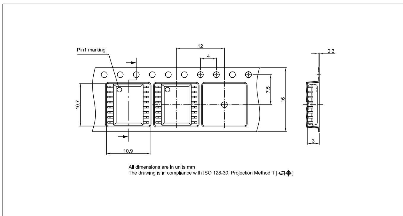
Figure 23 DSO16-300mil packing
