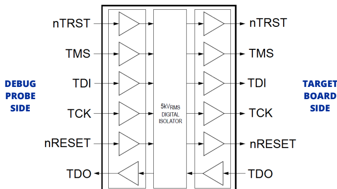
Isolated JTAG Signal Block Diagram
