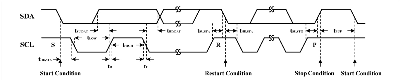
Figure 4 Interface Timing
