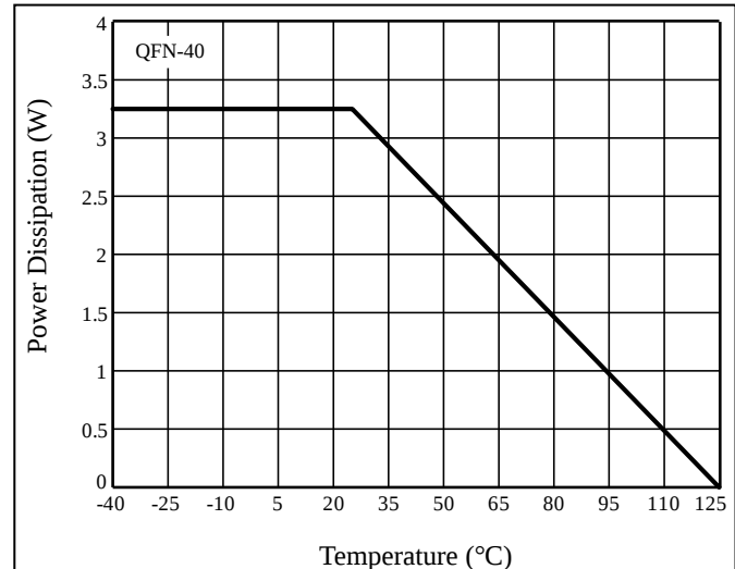
Figure 17 Dissipation Curve
