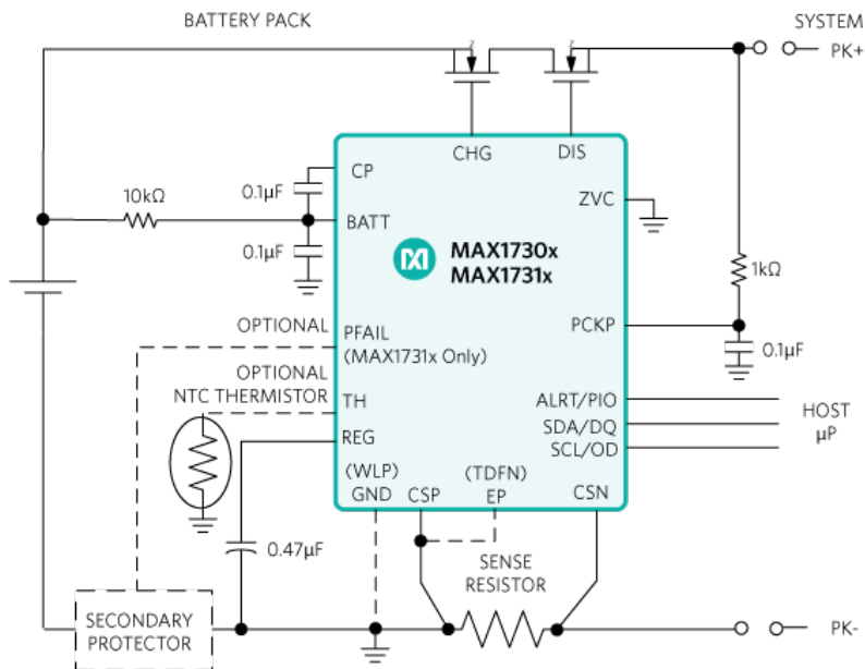
Figure 2. Fuel gauge and protection IC.
