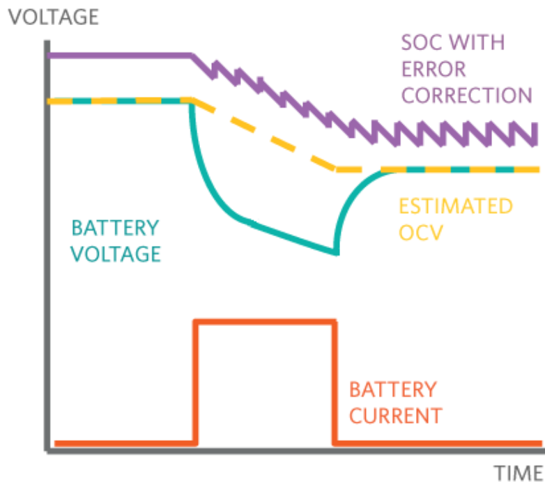
Figure 4. Accurate fuel gauging with ModelGauge M5.
