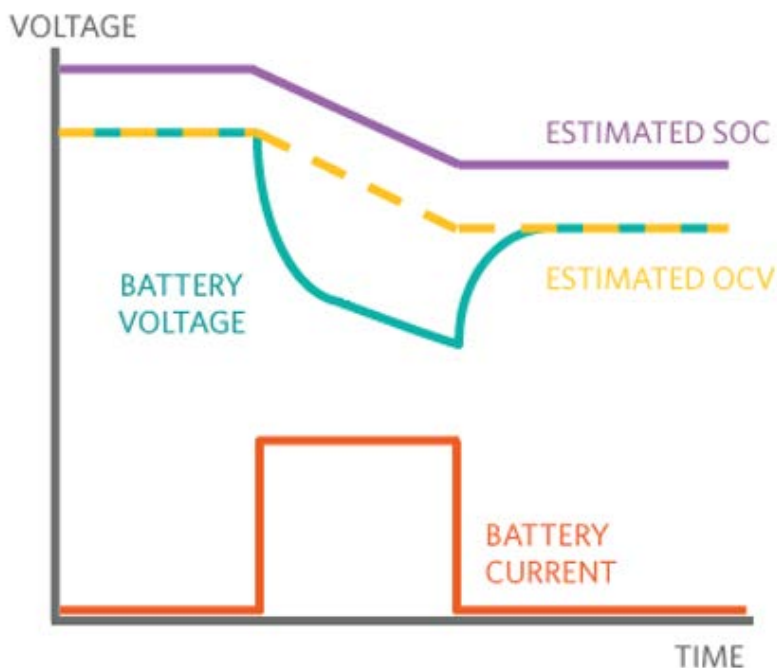
Figure 3. Voltage-based fuel gauge.
