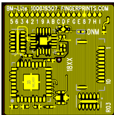
Figure 33. Example of PBC marking
