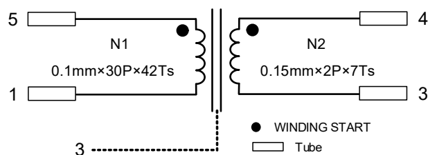
Figure 8: Electrical Diagram
