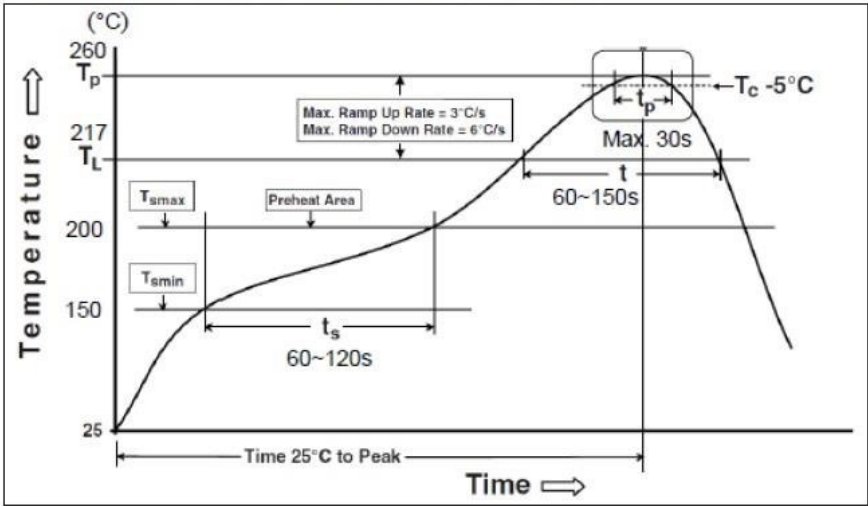
■Soldering Condition (Ref. IPC/JEDEC J-STD-020 & J-STD-002)
