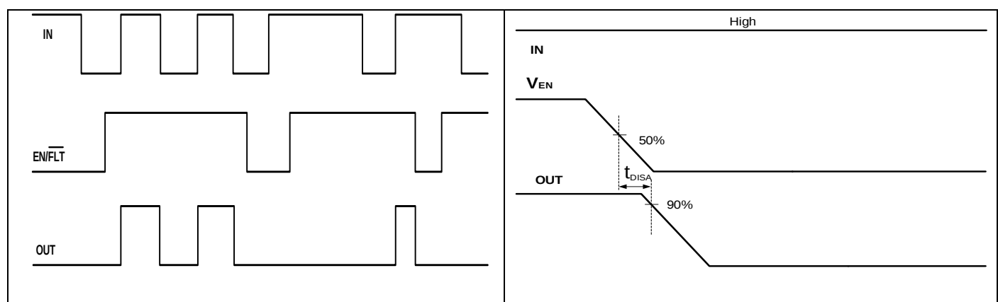
Figure 11 Input/output/enables pins timing diagram Figure 12 EN pin switching time waveform
