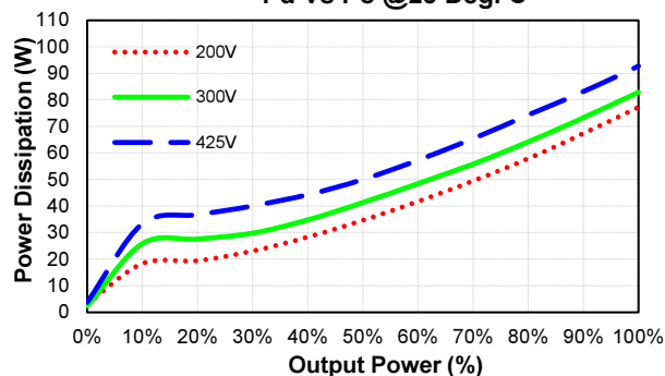
CFB750-300S28(N)-CMFD Pd Vs Po @25 Deg. C
