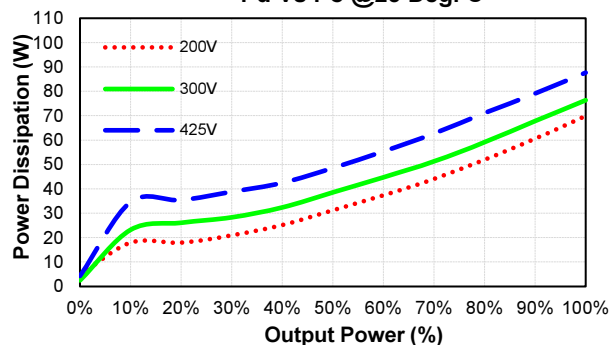
CFB750-300S36(N)-CMFD Pd Vs Po @25 Deg. C
