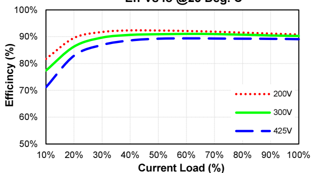
CFB750-300S24(N)-CMFD Eff Vs Io @25 Deg. C
