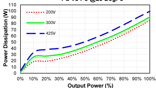
CFB750-300S15(N)-CMFD Pd Vs Po @25 Deg. C
