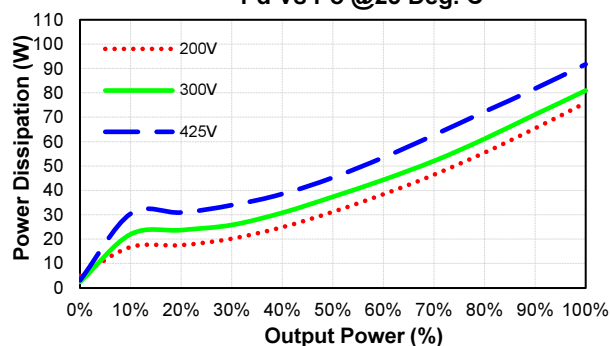
CFB750-300S24(N)-CMFD Pd Vs Po @25 Deg. C
