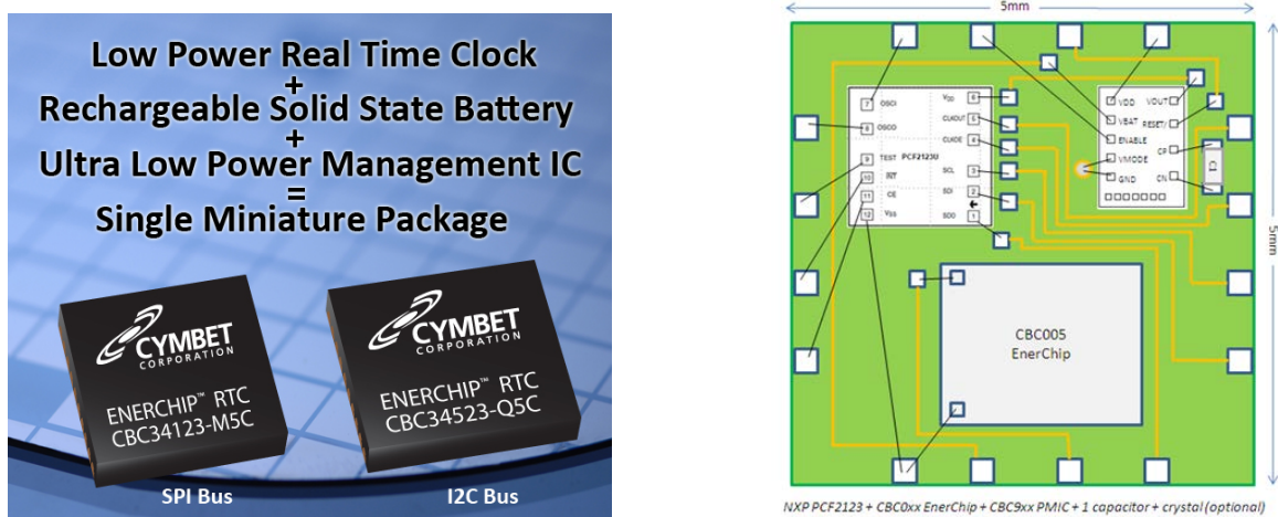
Figure 6: EnerChip Bare Die Integration in the Cymbet CBC34123 RTC with Integrated Battery
