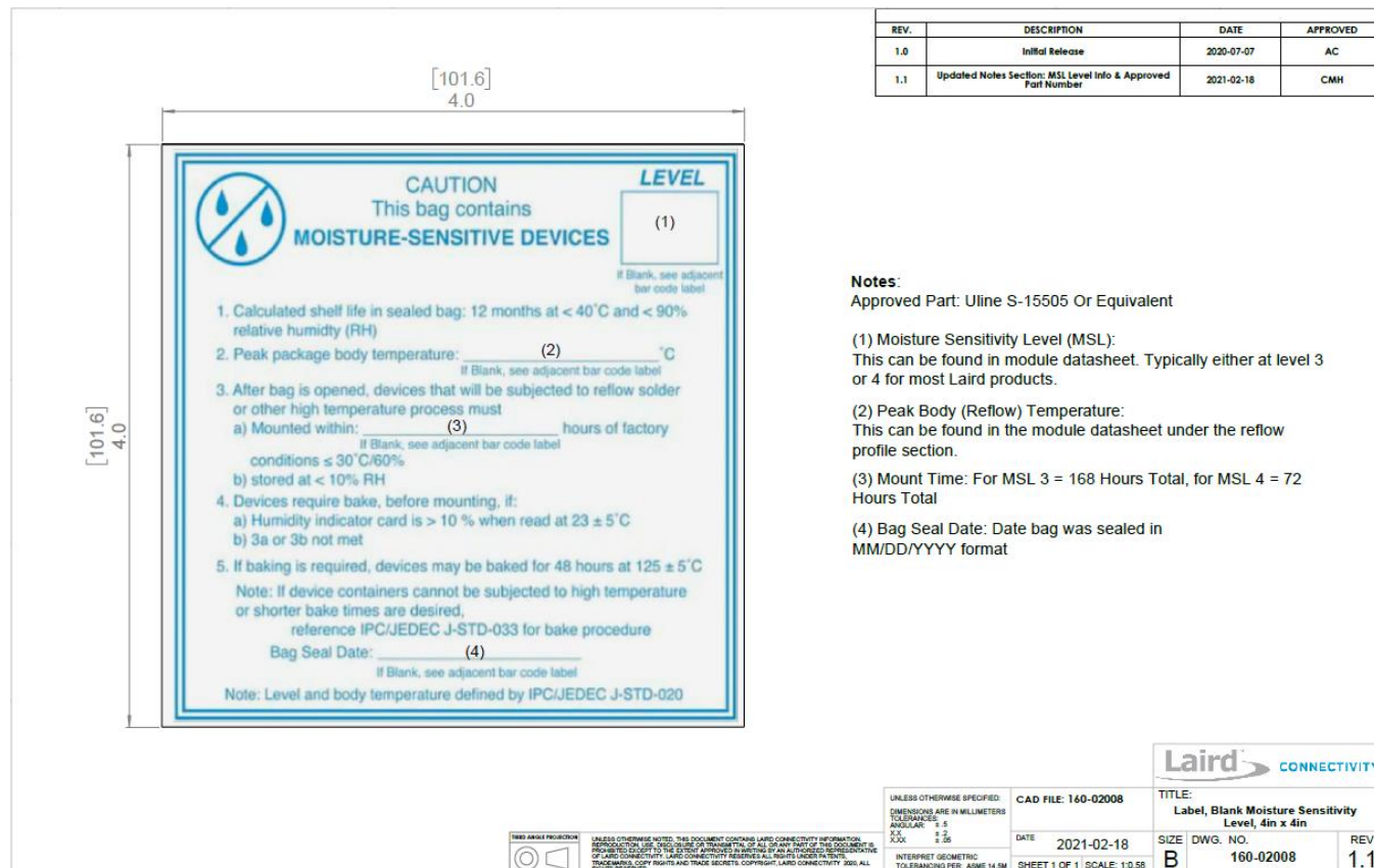
Figure 28: Sona IF573 Moisture Sensitivity Level Label, 160-02008
