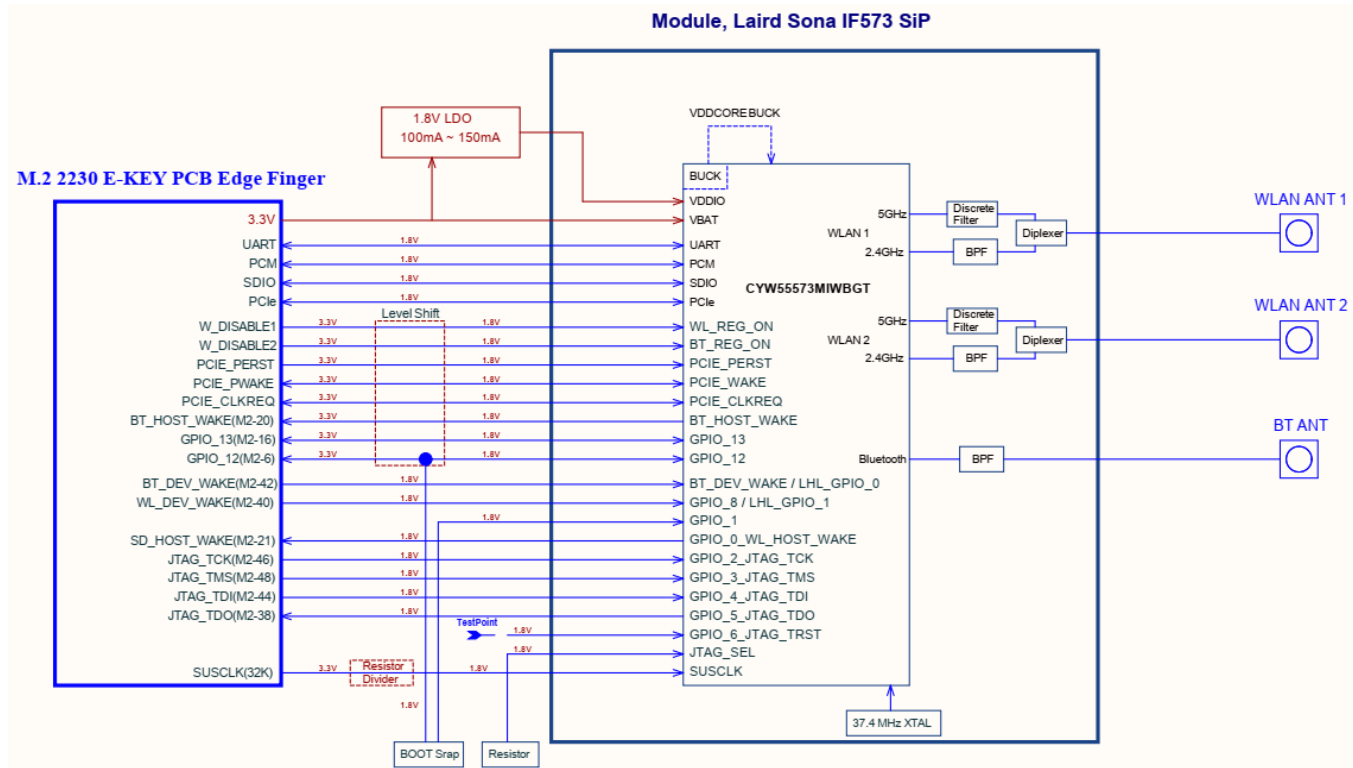
Figure 2: M.2 2230 E-Key
