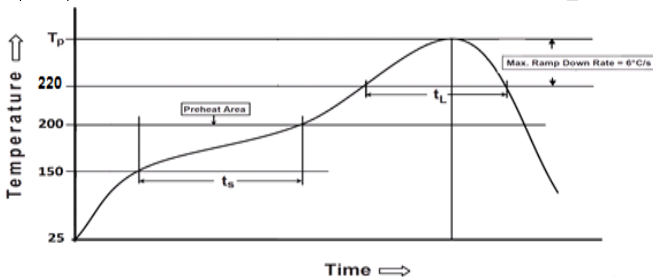
Figure 38: Temperature profile
