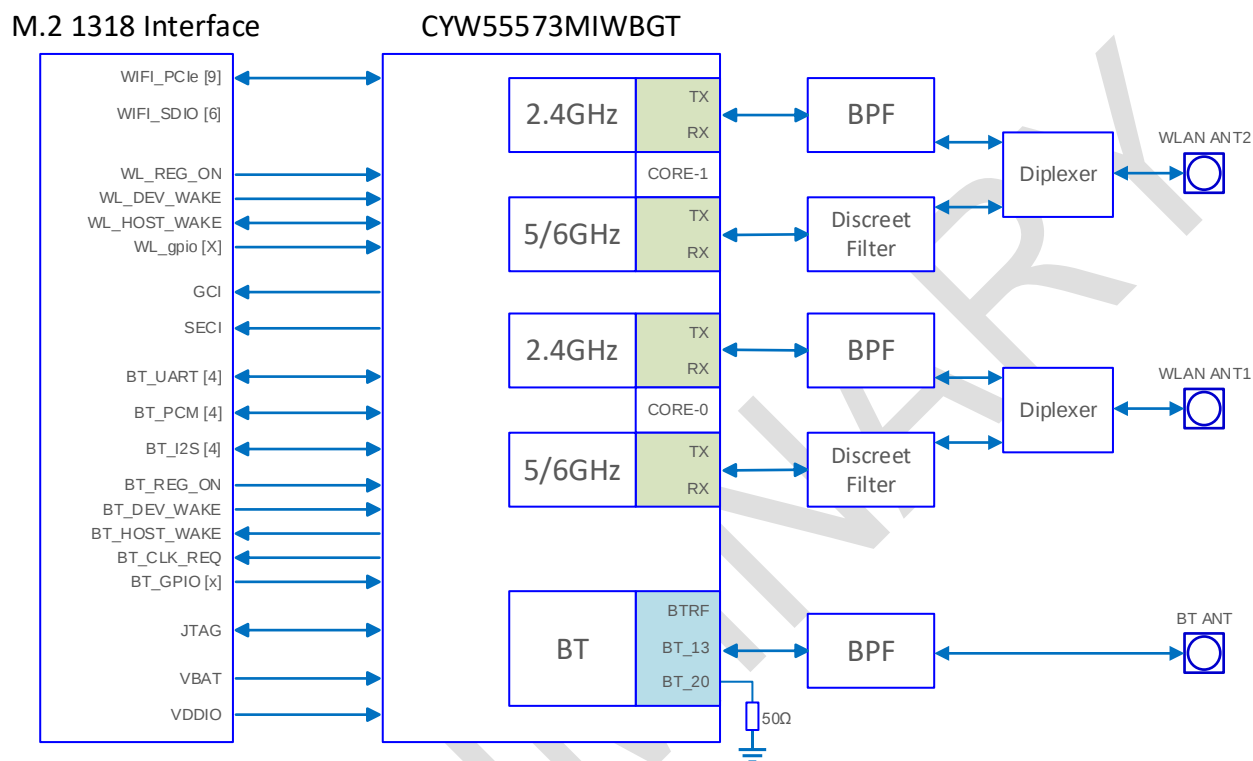
Figure 1: M.2 1318
